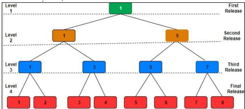
Figure 6. Minimax Algorithm
