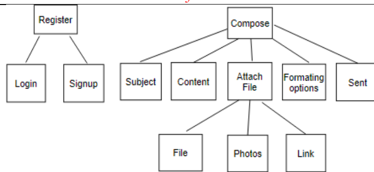
Figure 7. Requirements Tree I
