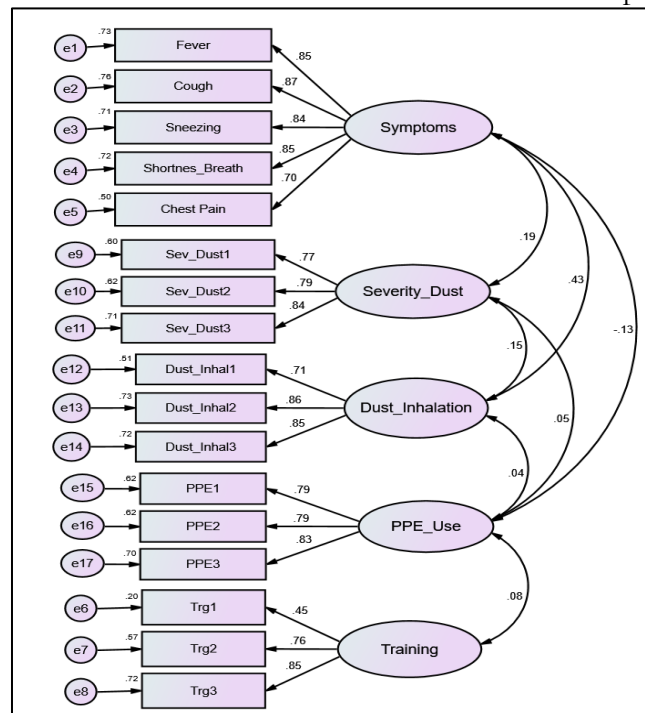
Figure 10: Measurement Model
