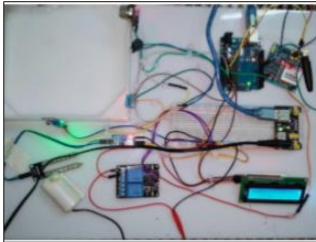
Figure 5. Hardware components
