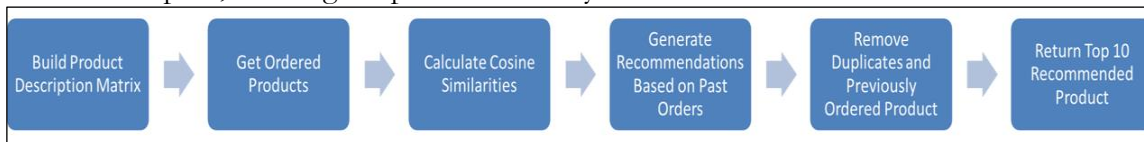
Figure 1. Content-Based Filtering
