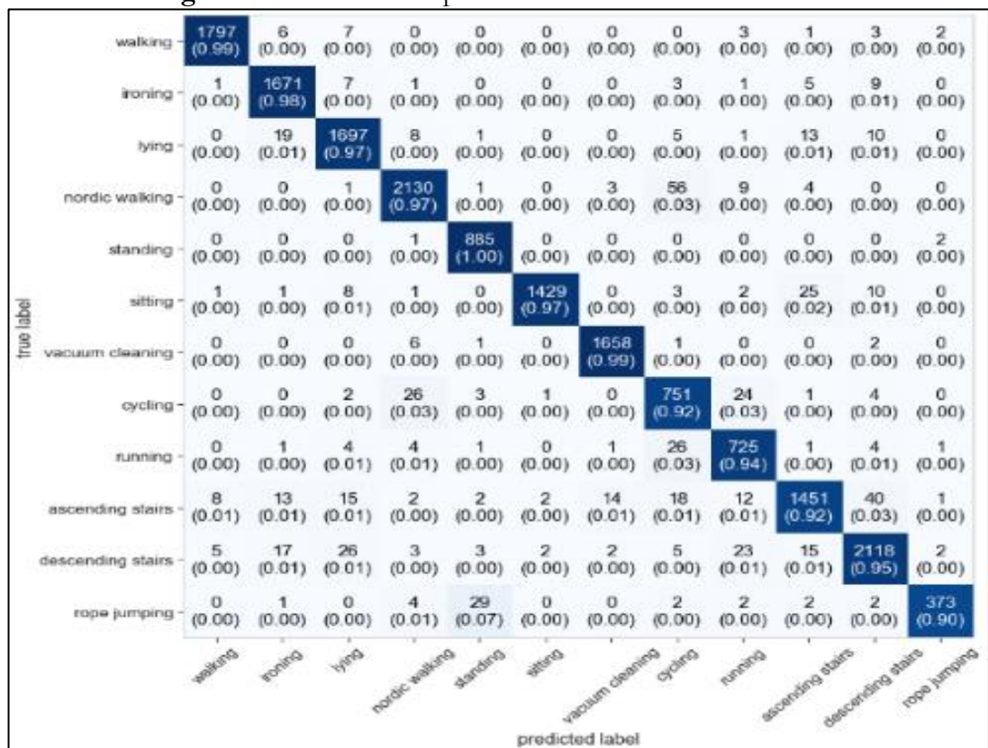
Figure 6. Confusion matrix and evaluation graph of PAMAP2
