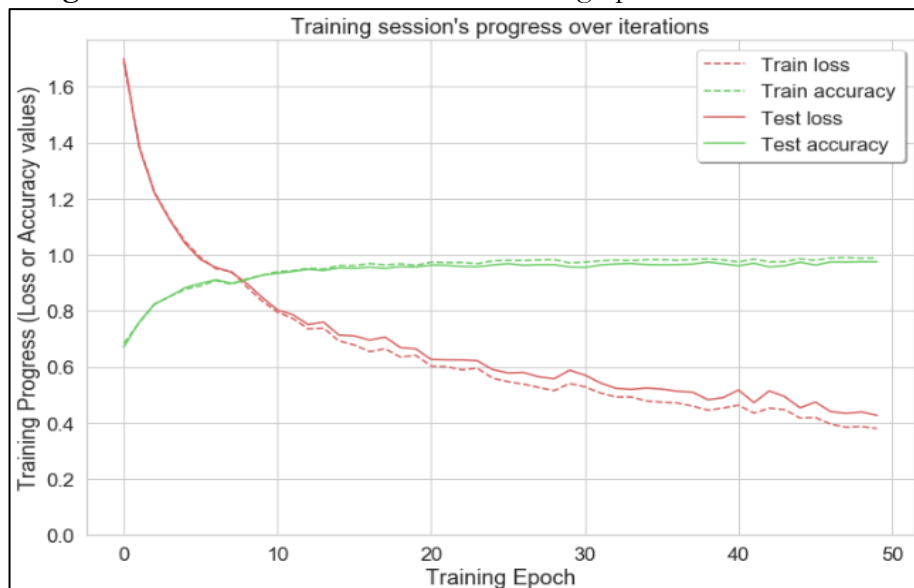
Figure 10. Evaluation graph of Wismd Human Activities Dataset
