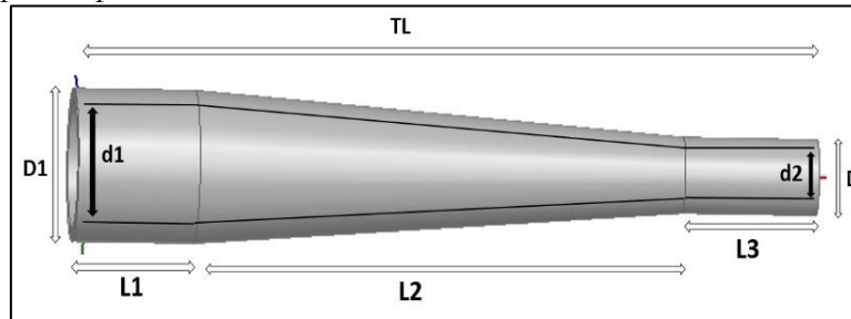
Figure 2. Description of the dielectric part of the antenna
