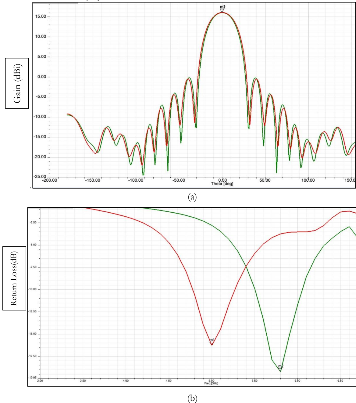
Figure 4. (a) Gain comparison with different materials of Yagi PCB like FR4 Epoxy (4.4) and FBR (2.55) (b) Frequency comparison with different materials of Yagi PCB like FR4 Epoxy (4.4) and FBR
