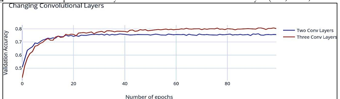
Figure 7. CNN - Impact and Analysis Changing Convolutional Layers
