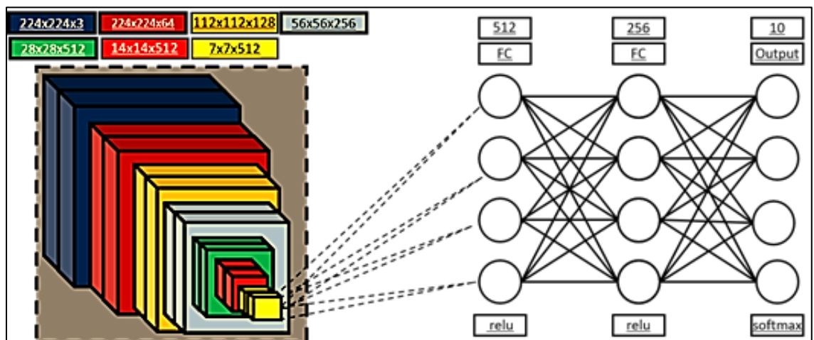
Figure 3: Transfer Learning using VGG-16 architecture
