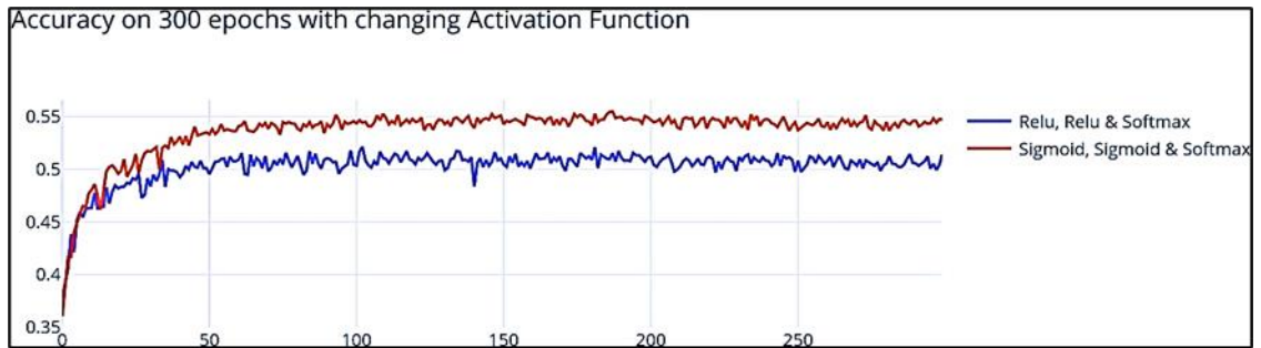
Figure 4. MLP - Accuracy on 30 epochs with changing Activation Function
