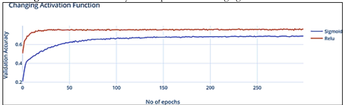
Figure 5. CNN - Accuracy on 30 epochs with changing Activation Function
