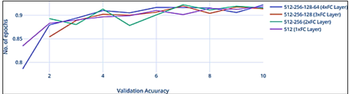
Figure 8. CNN - Impact and Analysis Changing Convolutional Layers
