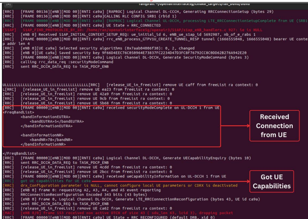
Figure 7. eNodeB showing communication between UE and eNodeB
