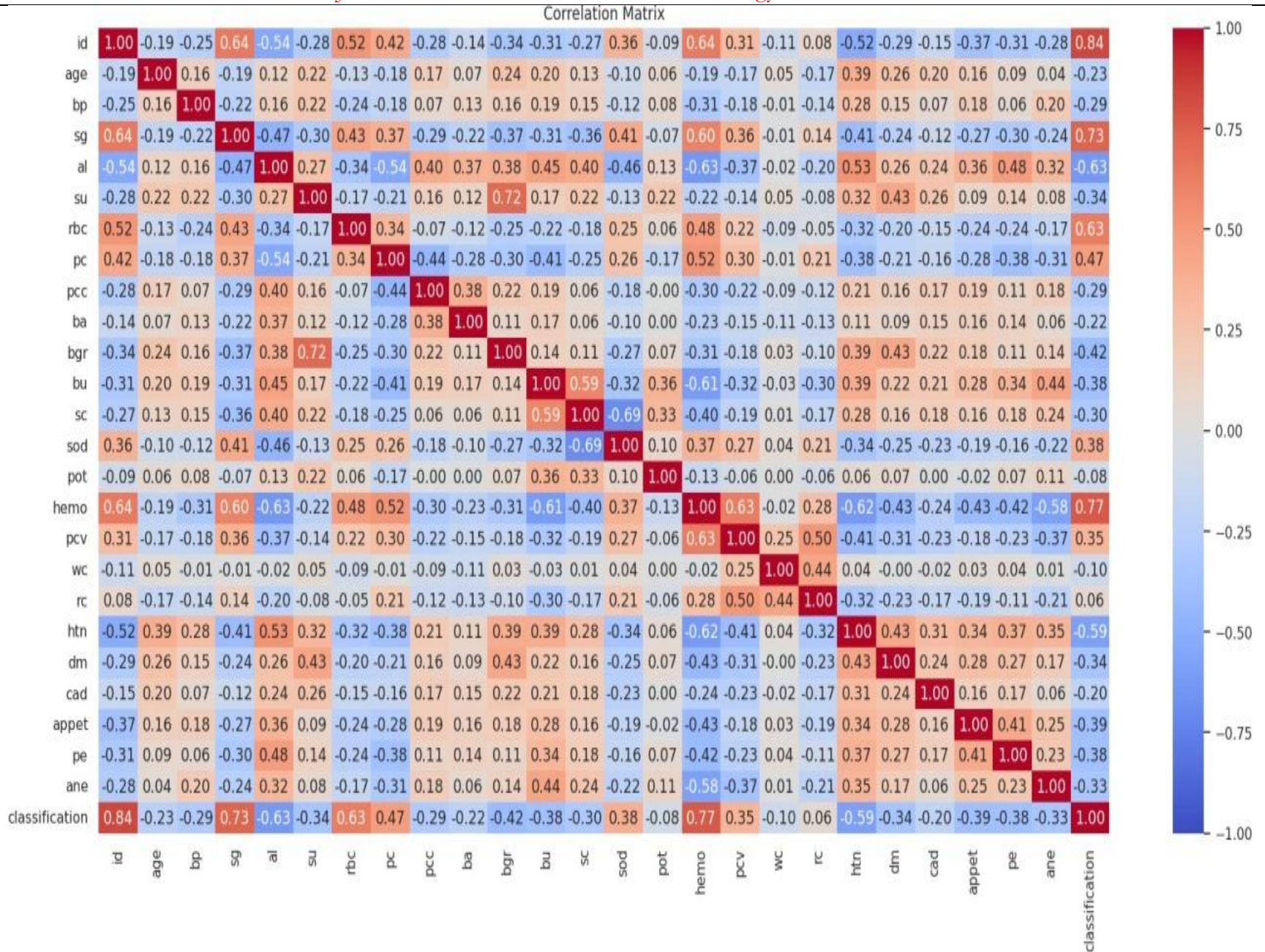
Figure 5. Correlation Matrix
