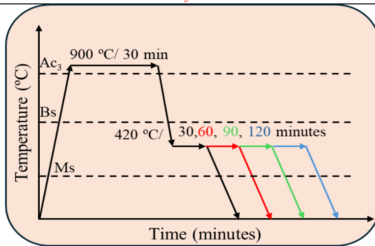
Figure 1. Austempering heat cycle adopted for experimental steel.
