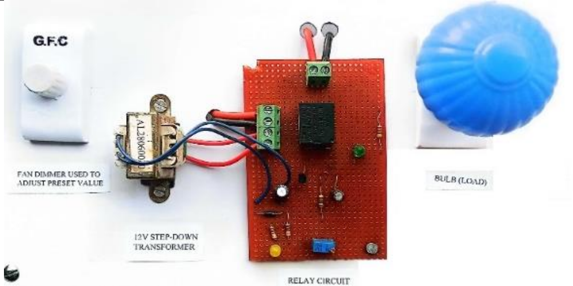
Figure 6. Hardware implementation before connection.
