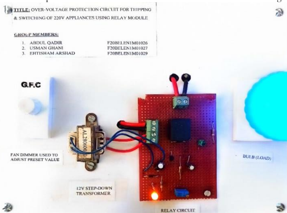
Figure 7. Hardware implementation after connection.
