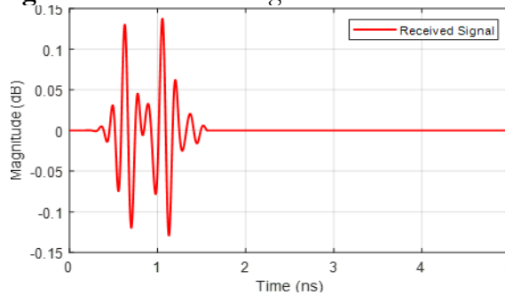
Figure 9. Received signal of MAVA antenna
