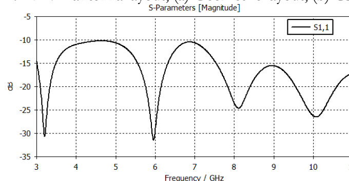
Figure 3: Reflection coefficient S_{11} of MAVA
