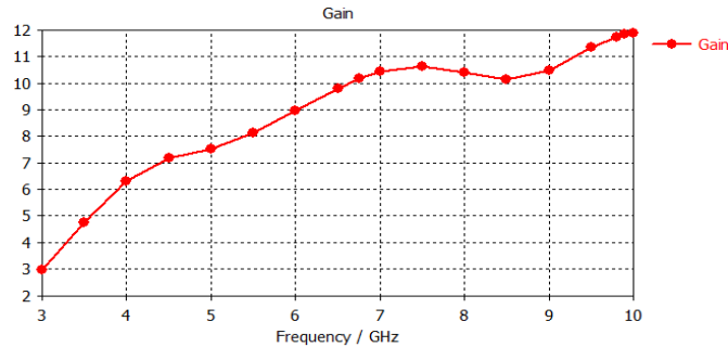
Figure 6. Simulated gain of MAVA (3-10 GHz)
