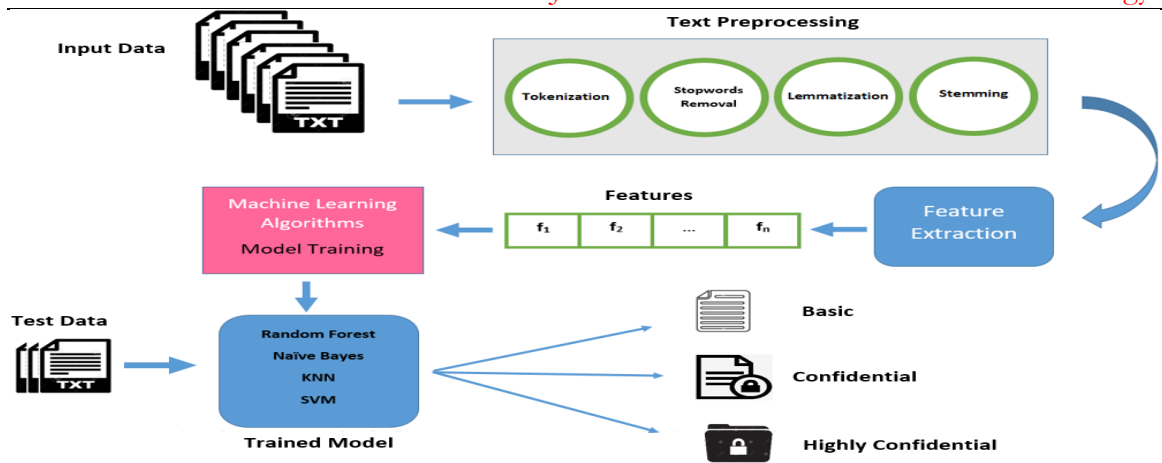
Figure 3. Proposed Automatic Data Classification Framework for Cloud Computing
