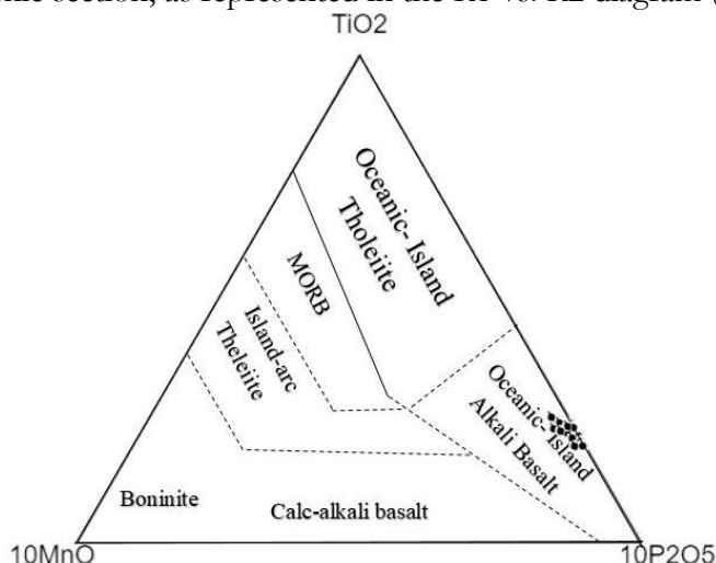
Figure 10. Show the studied rocks classify within the field of ocean island alkali basalt of 10 MnO - TiO_2 - 10P_2O_5 plot [12].
