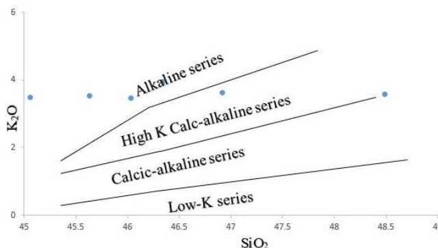
Figure 9. Shows that the mineralized zone has a high amount of potassium oxide thus these rocks act as an alkaline series after the SiO_2 - K_2O Plot [11].
