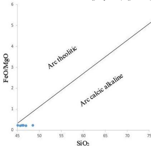
Figure 12. Mineralized rock samples fall in the field of Arc calcic alkaline in the \text{SiO}_2 - \text{FeOt/MgO} Plot [14].
