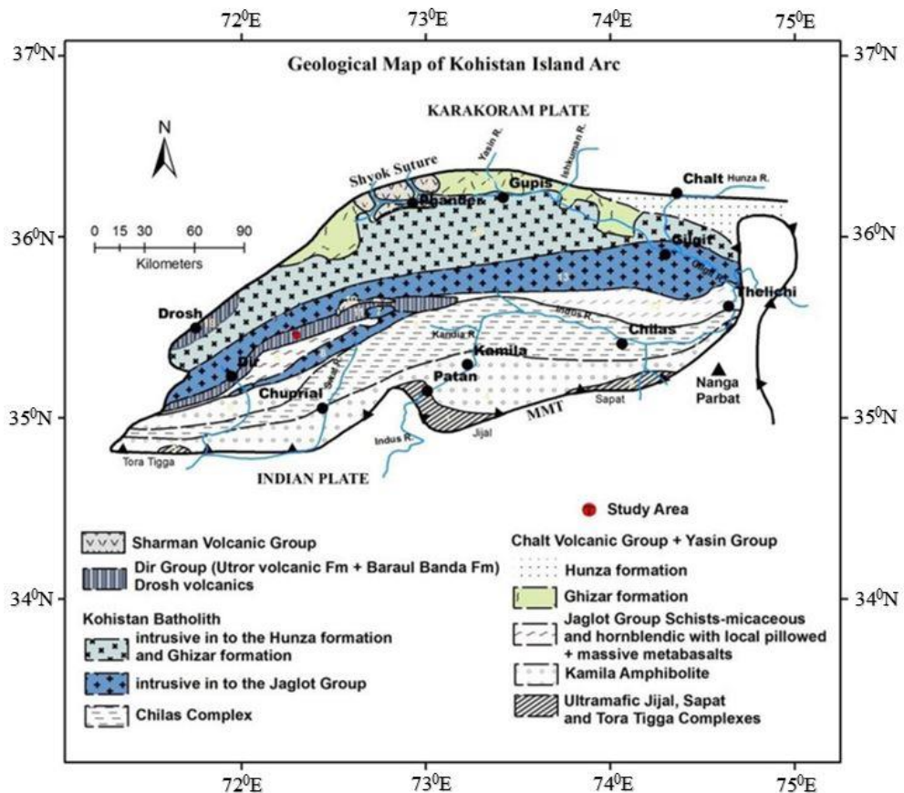
Figure 1. Geologic map of Kohistan Island Arc [8], the Red circle indicates the study area. Fieldwork:
