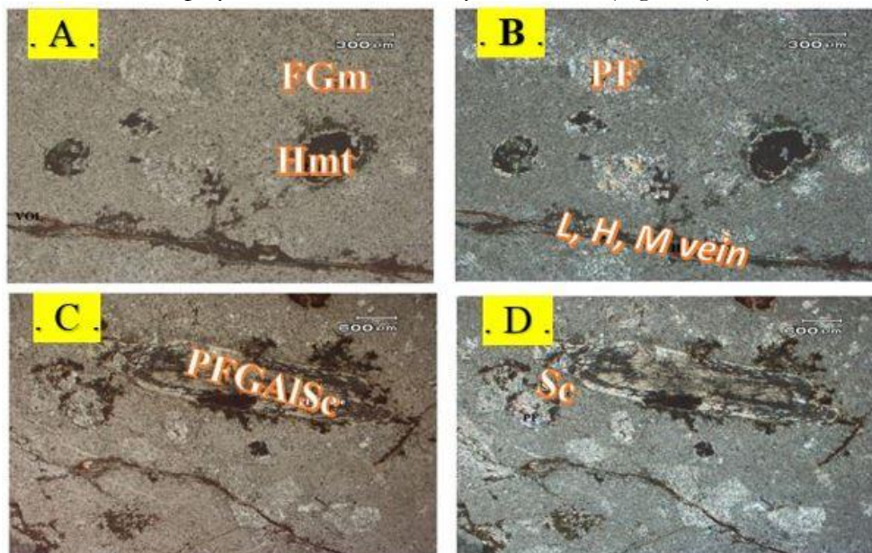
Figure 4. Photomicrographs (A, C XPL: B, D PPL) FGm-Fine groundmass, Hmt-Hematite, PF-Plagioclase feldspar, L, H, M vein- a vein of limonite, hematite and malachite, PFGAlSc- plagioclase feldspar grain altered into sericite, Se-Sericite.
