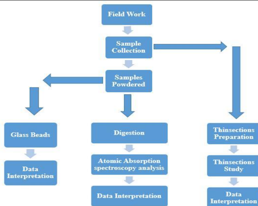
Figure 3. Flow diagram of methodology from fieldwork to data interpretation.
