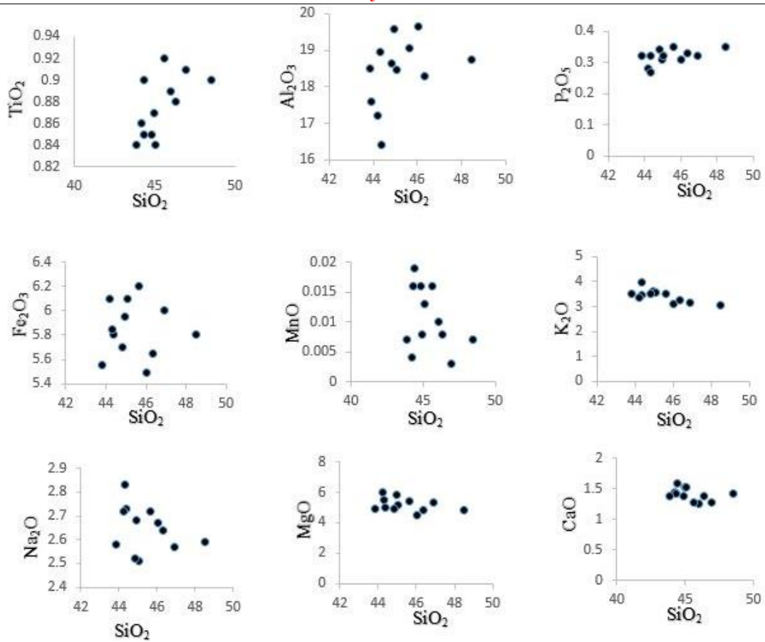
Figure 7. Shows binary plot of \text{SiO}_2 Vs \text{Na}_2\text{O} , \text{MgO} , \text{Al}_2\text{O}_3 , \text{P}_2\text{O}_5 , \text{K}_2\text{O} , \text{CaO} , \text{TiO}_2 , \text{Fe}_2\text{O}_3 and \text{MnO} [9].
