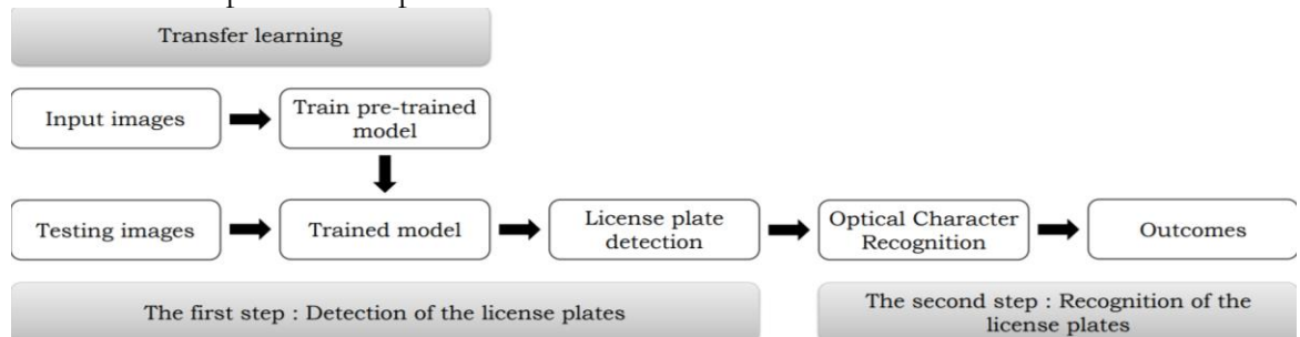
Figure 3. The diagram depicts the workflow of the proposed automatic license plate detection and recognition method, starting with license plate detection, followed by OCR-based character extraction, and ending with text output.
