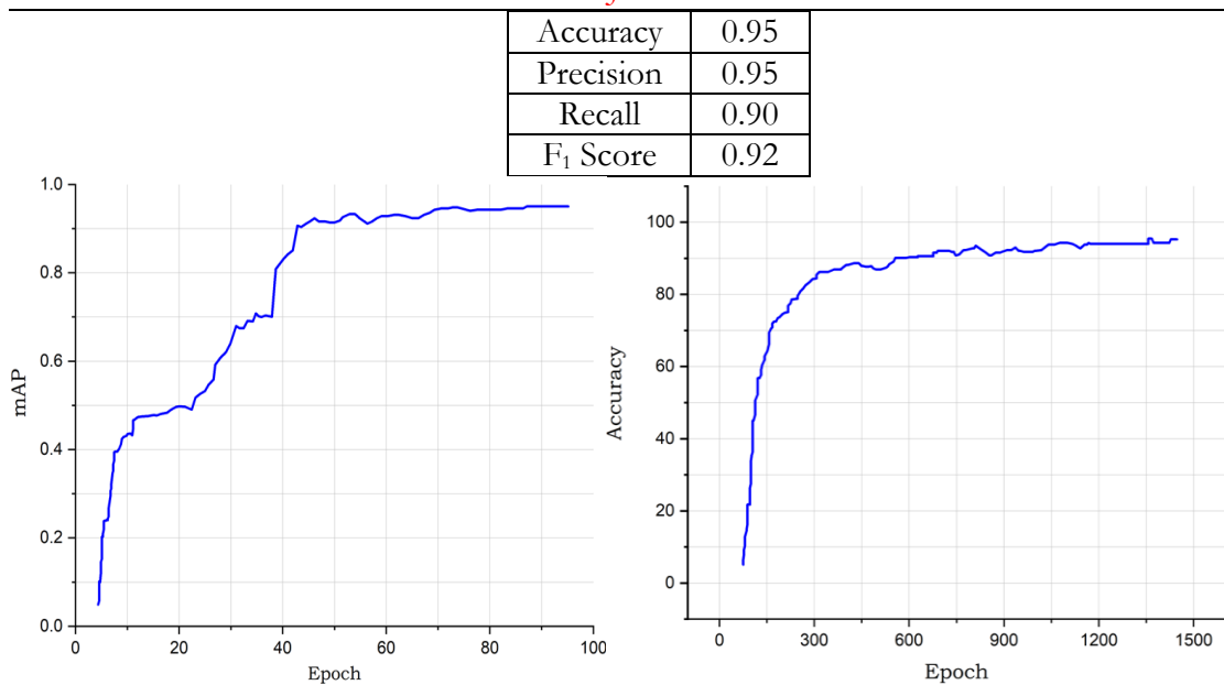
Figure 5. The performance metrics of the proposed algorithm. (a) shows the mean average precision (mAP) of 0.9418 on the testing dataset, demonstrating the model's performance in number plate detection and recognition, and (b) shows the model's accuracy of 95%, emphasizing its effectiveness in correctly detecting number plates.
