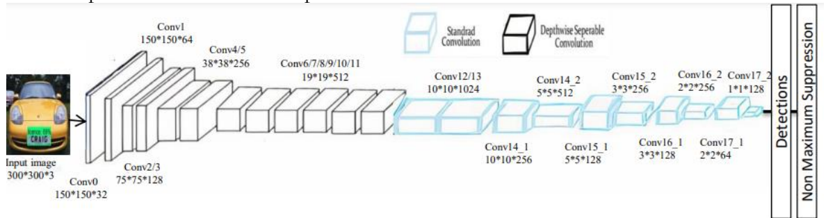
Figure 4. The architecture of the deep Mobile Net-SSD network comprises 22 convolutional layers, specifically designed to enhance detection capabilities. It includes 13 depthwise separable layers that optimize feature extraction efficiency and 9 standard convolutional layers utilized in object detection.
