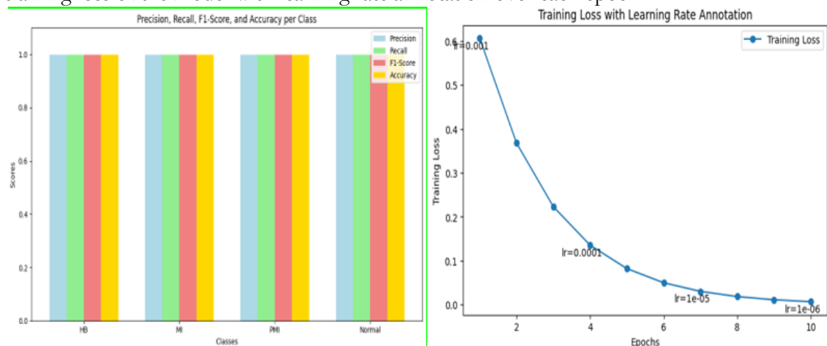
Figure 13. (a) Accuracy, Precision, Recall, and F1-score for each class. (b) Training loss with learning rate annotation.
