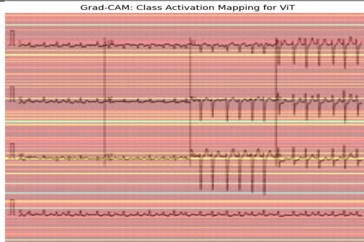
Figure 4. Grad-Cam: class activation mapping for ViT (to show parts of the ECG image model focused on for making predictions).
