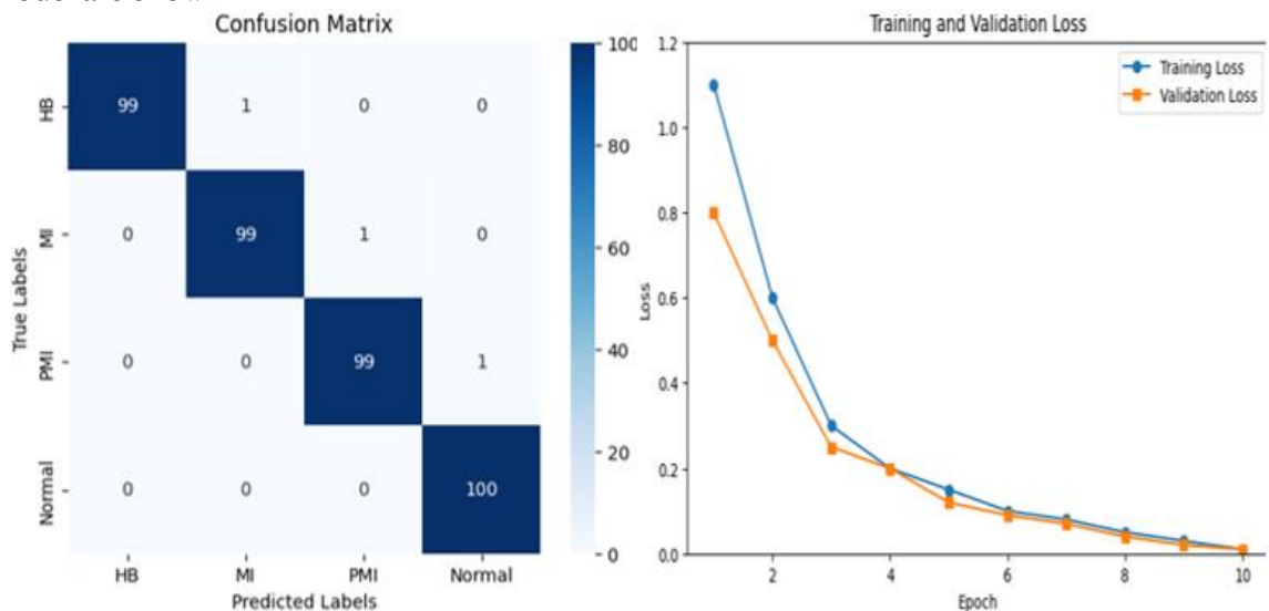
Figure 8. (a) Confusion matrix for ViT. (b) Training and validation loss for ViT.
