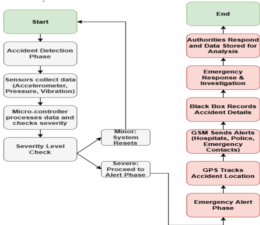
Figure 3: Methodology Flow Diagram of the Proposed ADRS
