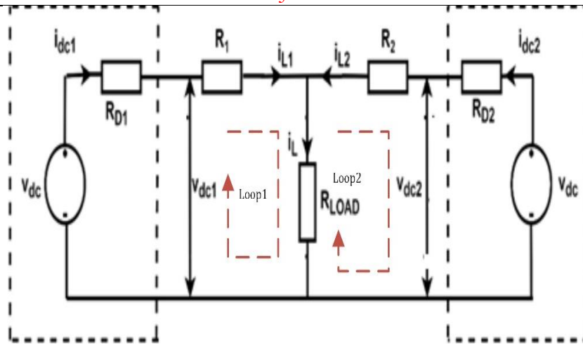
Figure 3 Steady-state equivalent circuit of two parallel connected sources.
