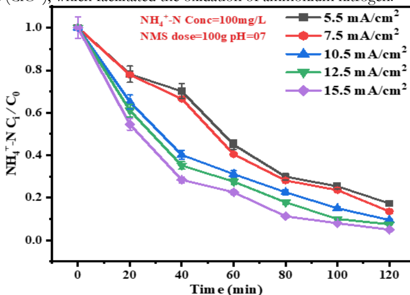
Figure 5. Current density vs. \text{NH}_4^+\text{-N} Removal Efficiency (%)
