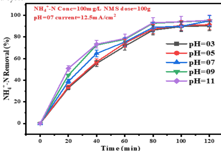
Figure 4. pH vs. \text{NH}_4^+\text{-N} Removal Efficiency (%)
