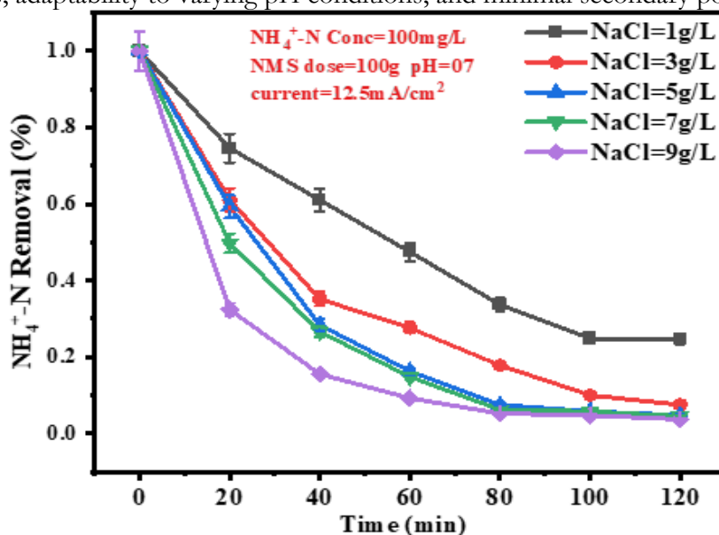
Figure 6. NaCl amount vs. \text{NH}_4^+ -N Removal Efficiency (%)
