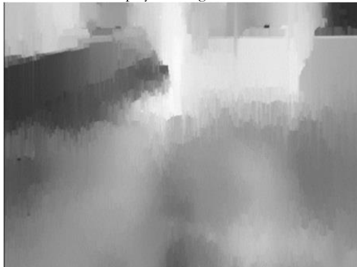
Figure 4. Disparity map
