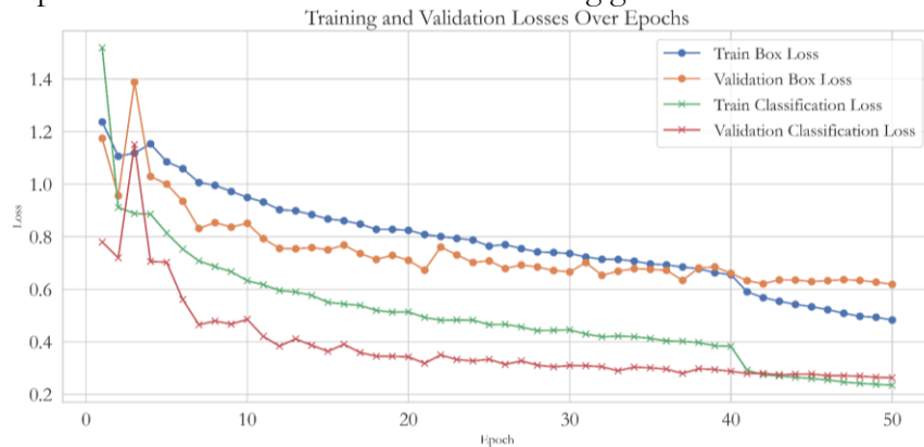
Figure 7 Training and validation losses show a steady decline, indicating effective learning with minimal overfitting, despite slightly higher validation losses
