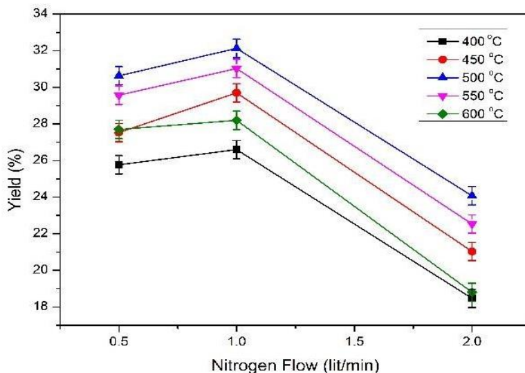
Figure 5. Nitrogen Flow's impact on Bio-oil Yield %
