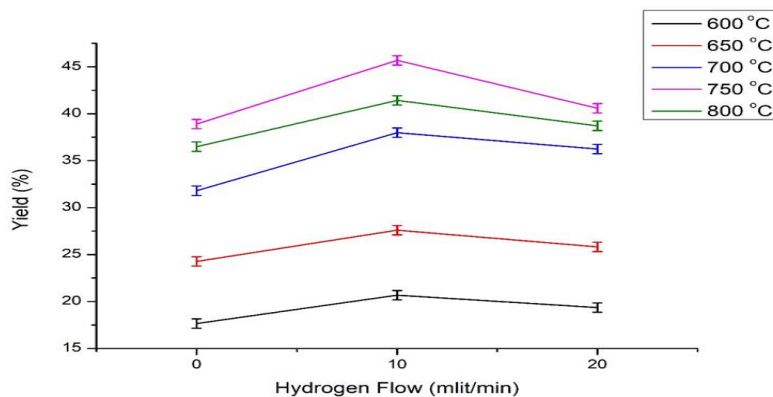
Figure 5. Effect of hydrogen composition in the Yield
