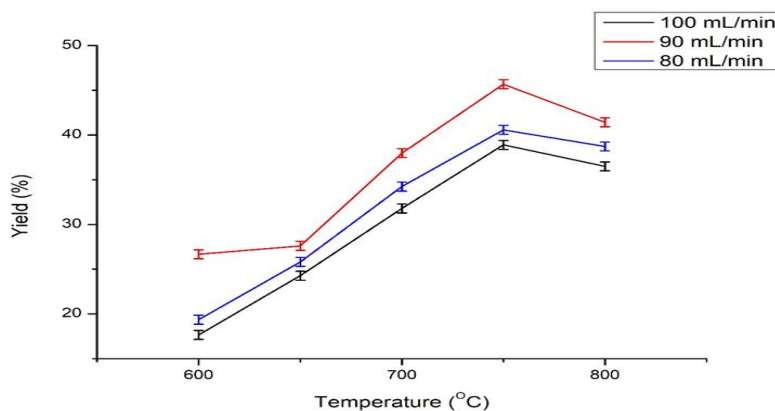
Figure 4. Effect of pyrolysis temperature in the Yield
