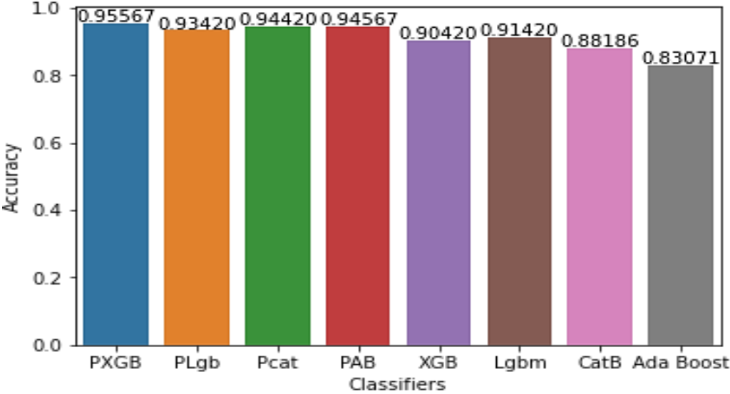
Figure 5. Accuracy report of various models
