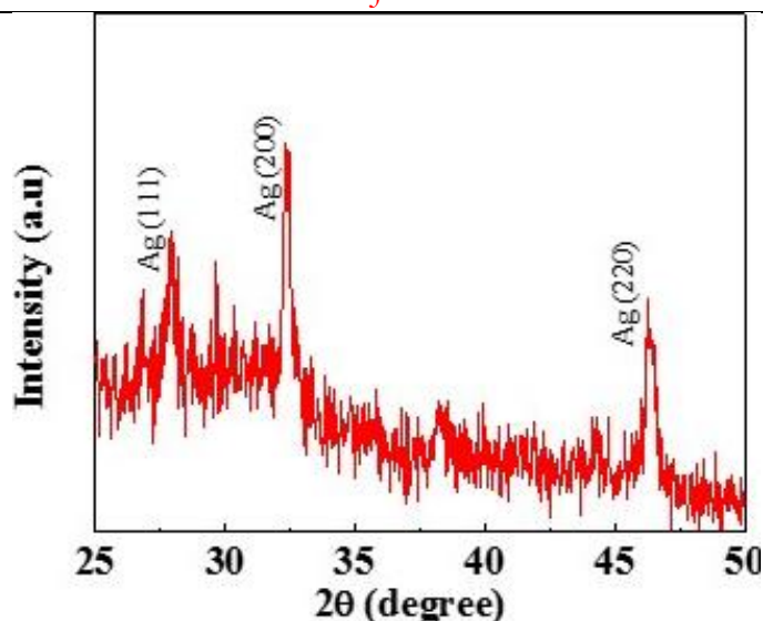
Figure 3. X-ray diffraction analysis of w2 shows the pattern formed by nanoparticles, indicating greater peaks at (2\theta) 27.98, 32.31, and 46.23 corresponding to (111), (200), and (220) respectively. The peak (200) shows particle size as 23 nm.
