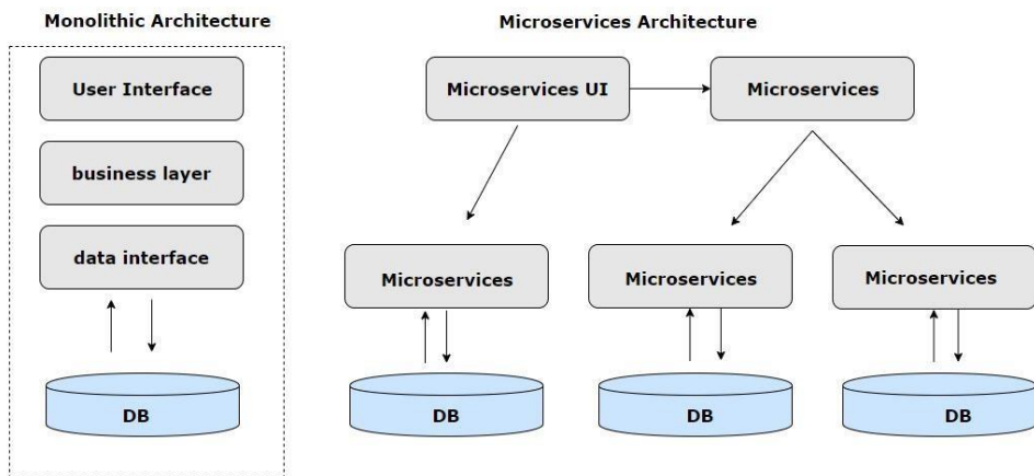
Figure 2. Microservices Architecture
