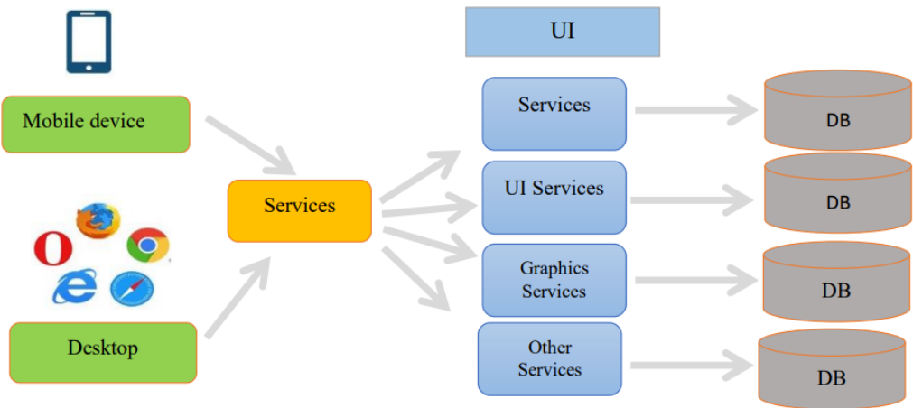
Figure 2. Microservices Architecture
