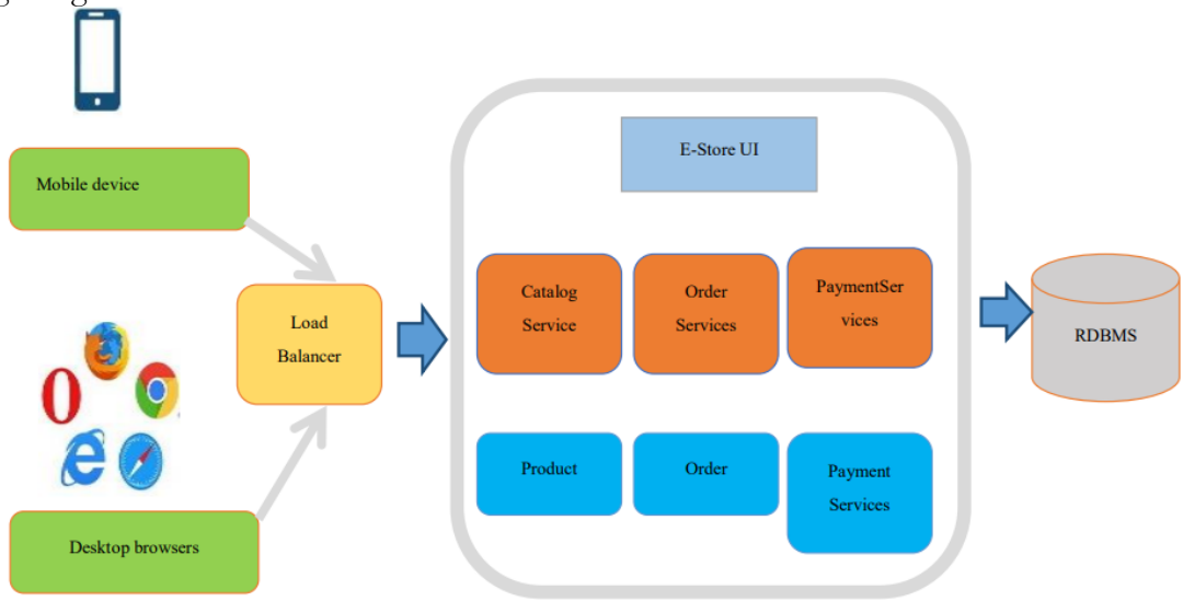
Figure 1. Monolithic Architecture
