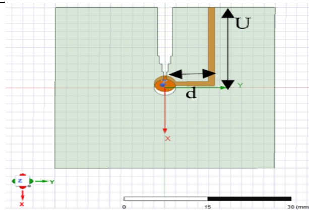
Figure. 2. Single Element of Linear Tapered Slot Antenna
