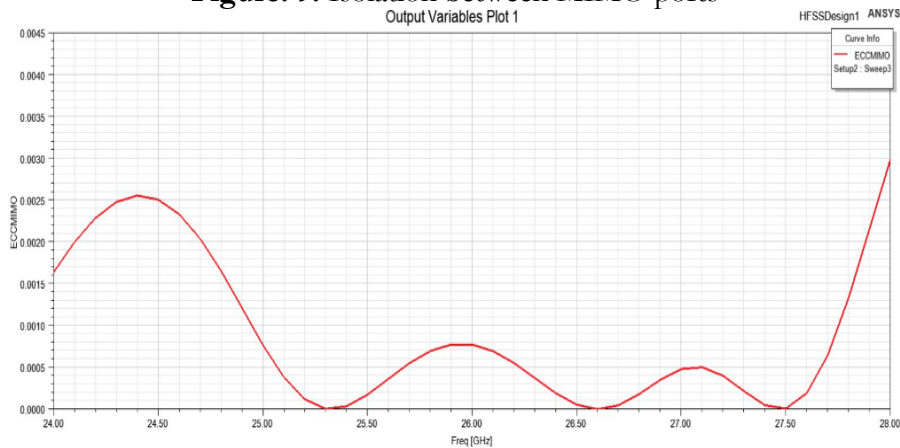
Figure. 10. Envelope Correlation Coefficient of MIMO Array
