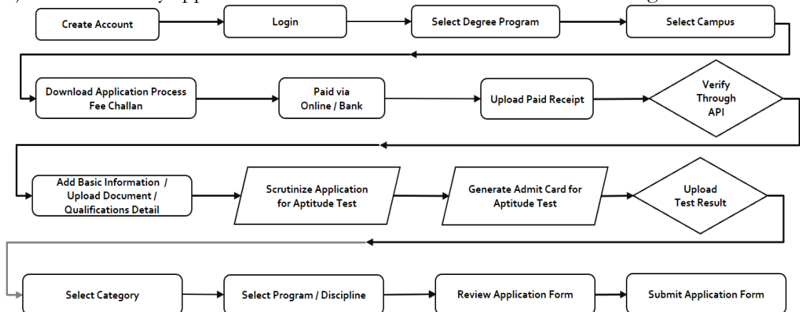
Figure 4. Data flow diagram of the proposed automated admission system Seat Allocation in the Proposed System:
