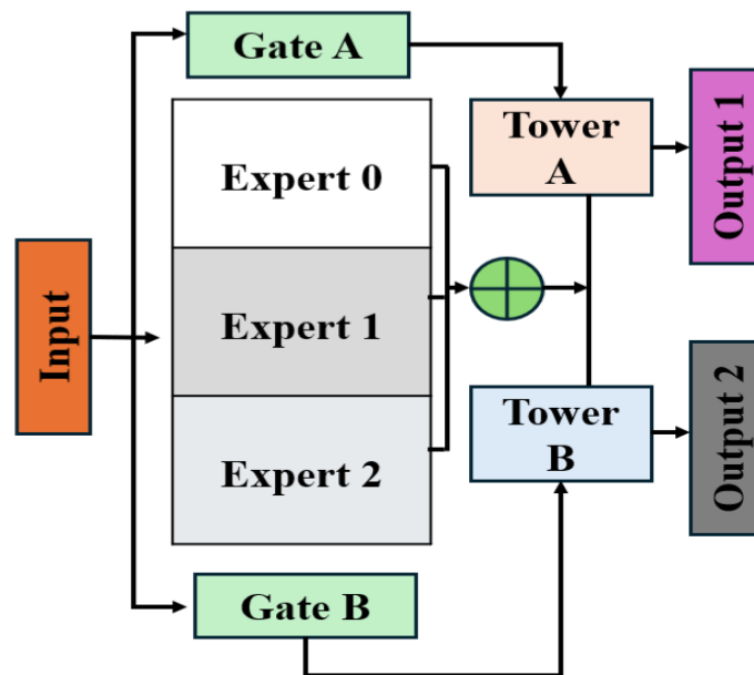
Figure 2. Framework for Multitask learning.
