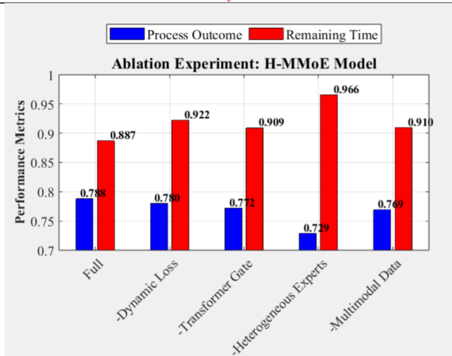
Figure 7. H-MMoE Model Ablation Experimental Result
