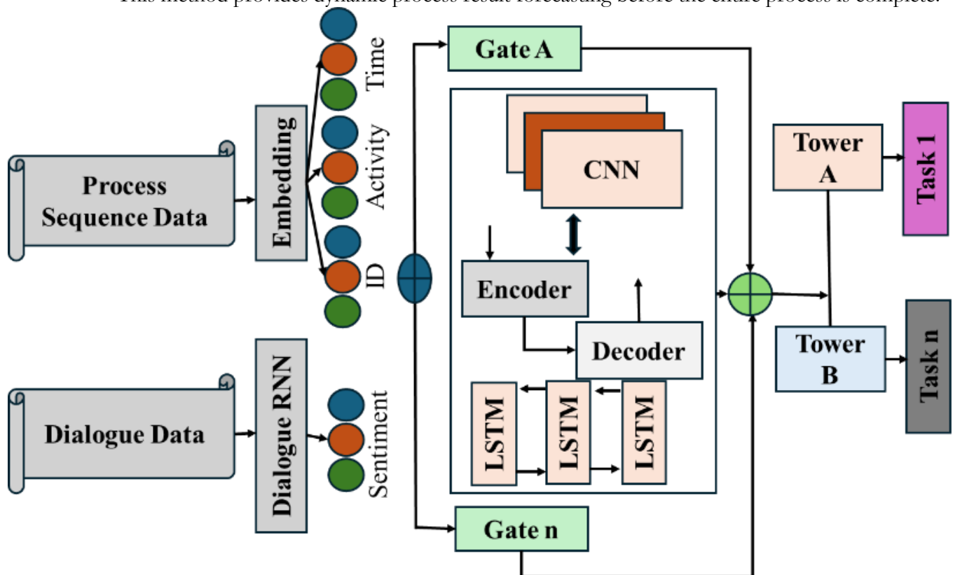
Figure 3. Proposed Methodology Framework.
