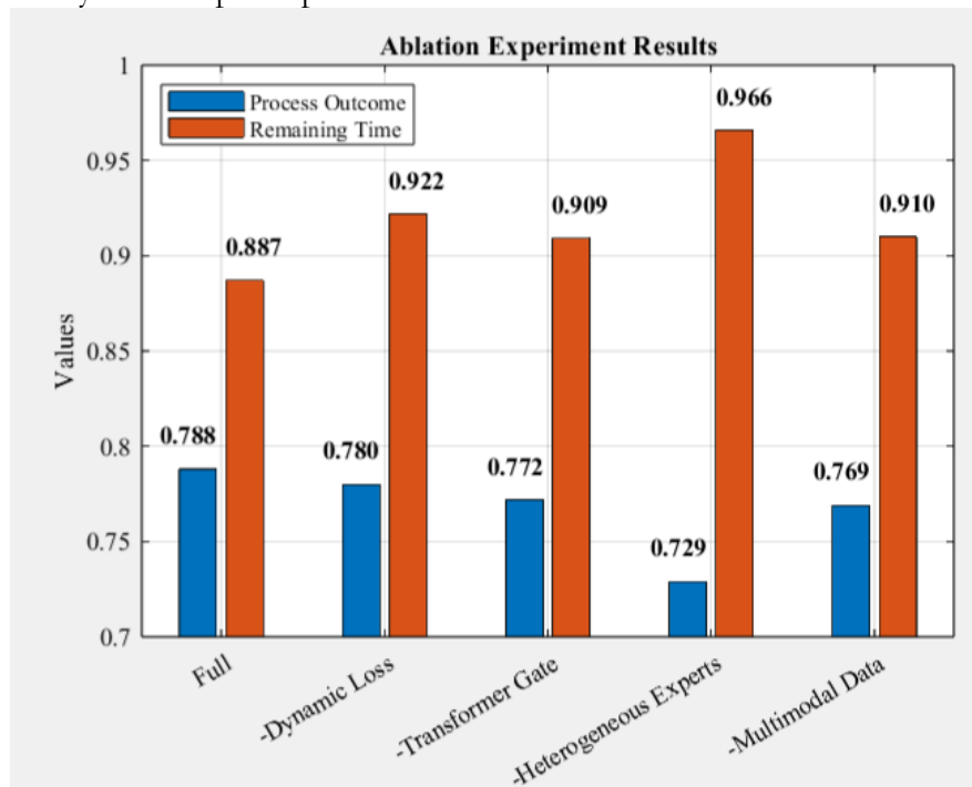
Figure 6. Ablation Experimental Results.
