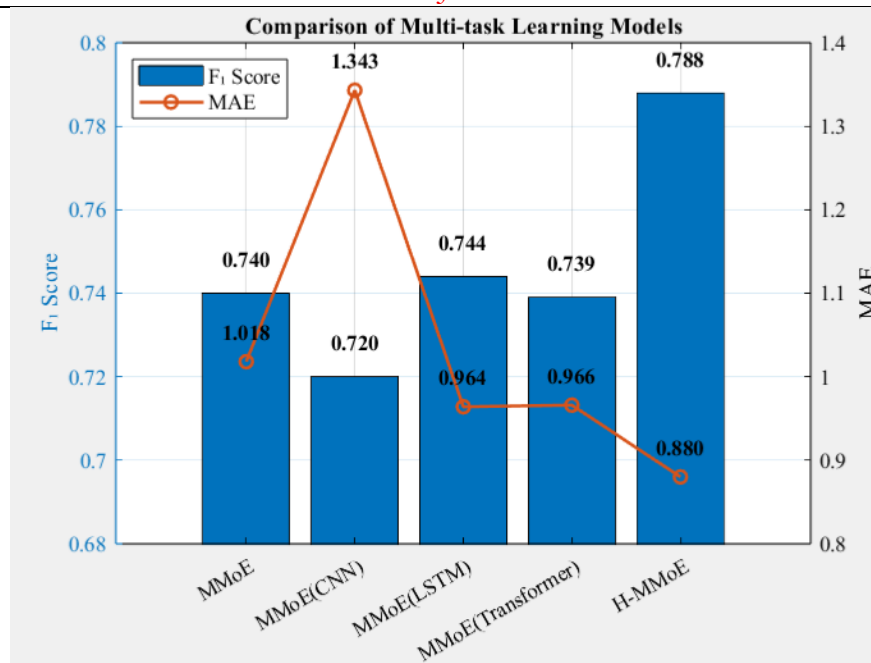
Figure 5. Multitask learning Results comparison.
