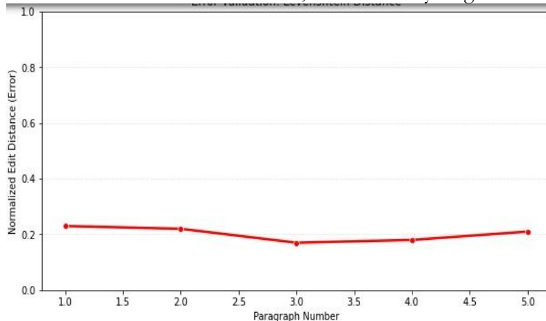
Figure 3. This graph for Error Validation Using Levenshtein Distance
