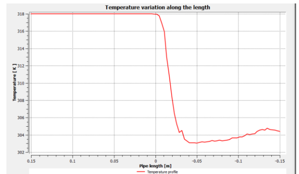
Figure 16. Temperature Profile for Case 3
