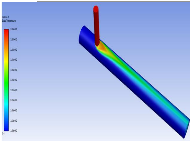
Figure 7. Circular T-junction temperature contour in 3D analysis
