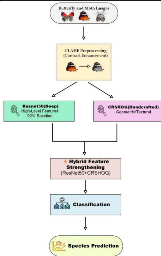
Figure 2. Flow diagram for Butterfly and Moth image classification
