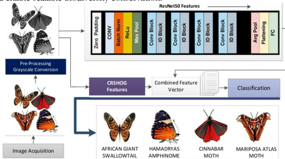
Figure 1. Workflow of the Proposed CRSHOG-ResNet50 Hybrid Methodology.
