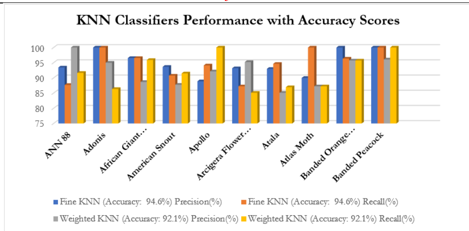
Figure 9. Comparison of Fine and Weighted KNN classifiers
