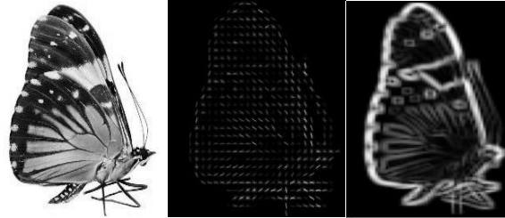
Figure 7. (a) Grayscale Image; (b) HOG Magnitude; (c) CRSHOG Magnitude.
