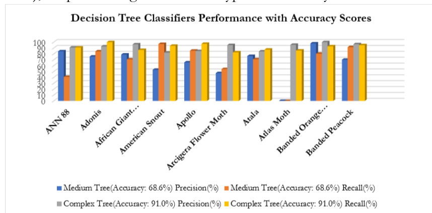
Figure 11. Performance comparison of Decision tree classifiers.
