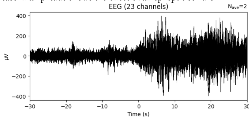
Figure 2. Seizure Epoch
