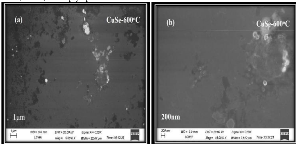
Figure 4. SEM images for CuSe-600°C thin film at 1 \mu m and 200nm resolutions
