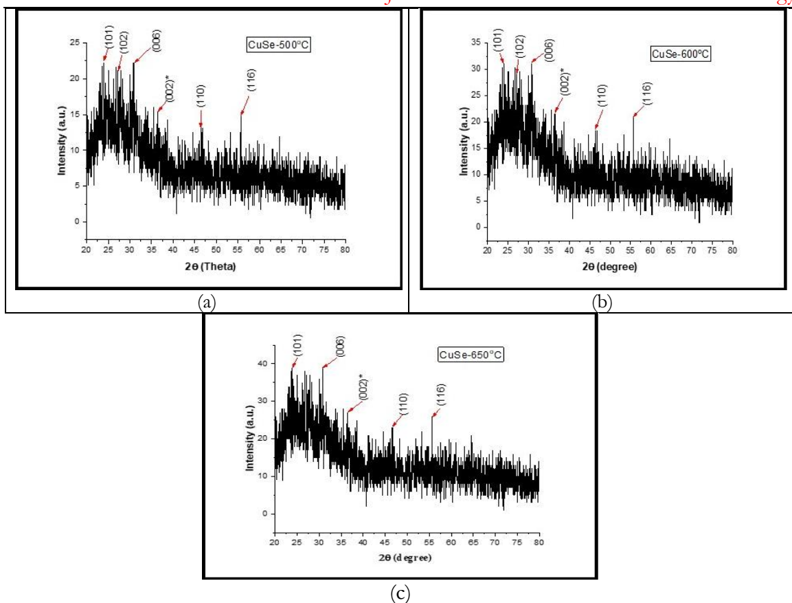
Figure 2. Represents the XRD patterns of CuSe-500 °C (a), CuSe -600 °C (b), and CuSe - 650 °C (c) thin films
