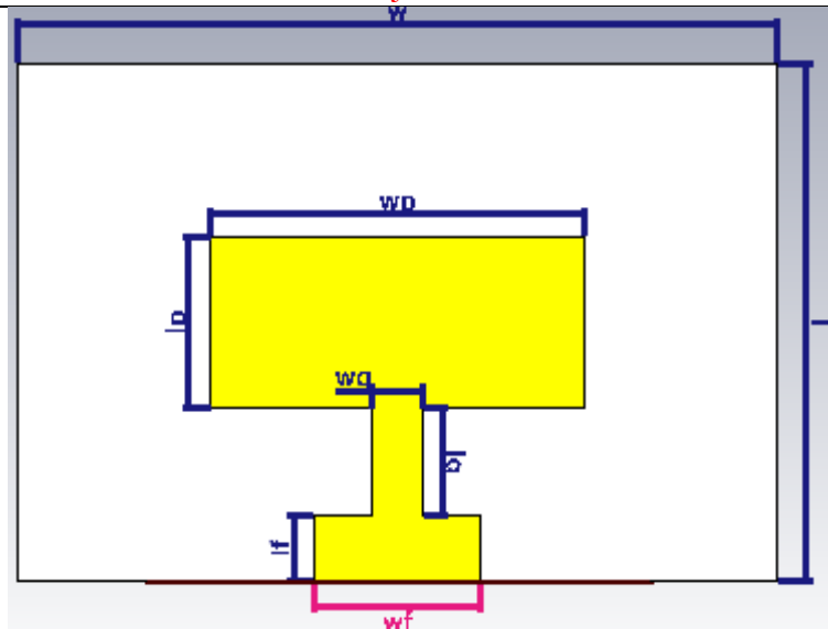
Figure 2. MPA with Feedline Technique
