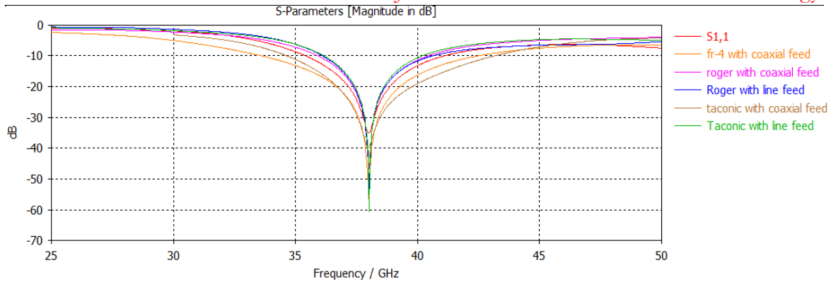
Figure 4. S-Parameters Comparison of different MPAs
