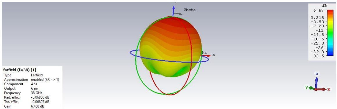
Figure 11. Gain of MPA with coaxial feed technique and Taconic RF-35C substrate
