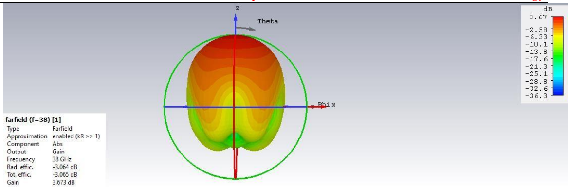
Figure 6. Gain of MPA with Line feed using FR-4 substrate. The gain is 3.67dB
