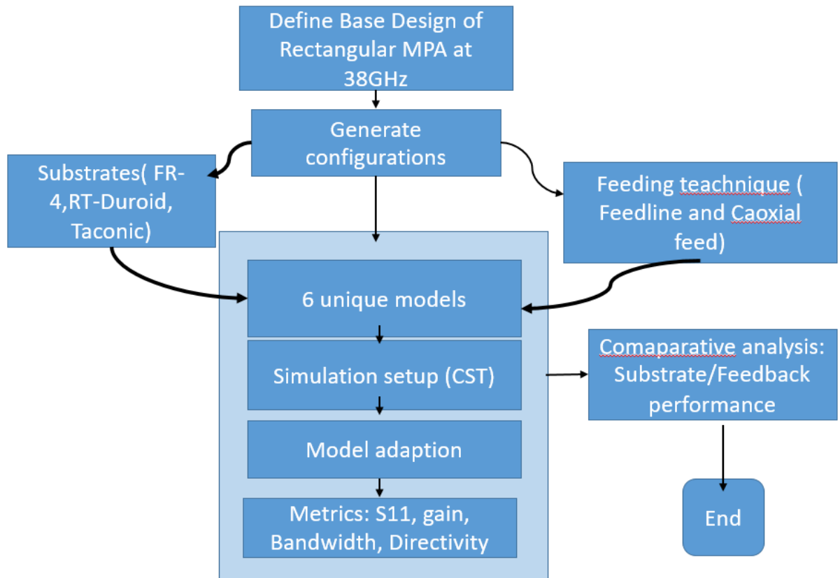
Figure 1. Workflow for 38 GHz MPA design, simulation, and performance comparison
