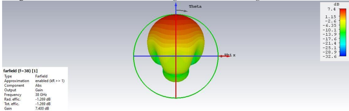
Figure 7. Gain of MPA with Line feed and Rogers RT Duroid substrate. The gain is 7.4dB
