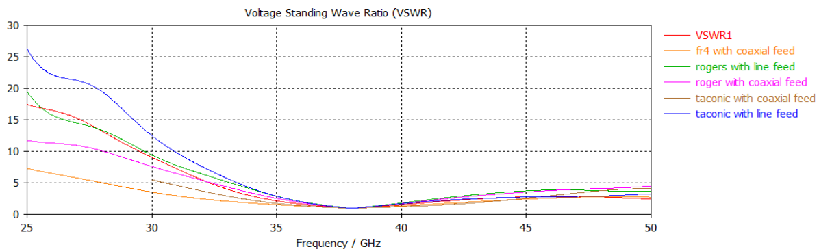
Figure 5. VSWR Comparison of different MPAs
