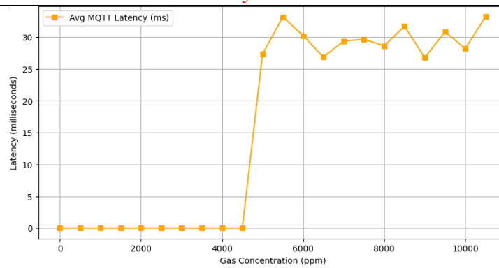
Figure 15. Average MQTT Message Latency vs. Gas Concentration.
