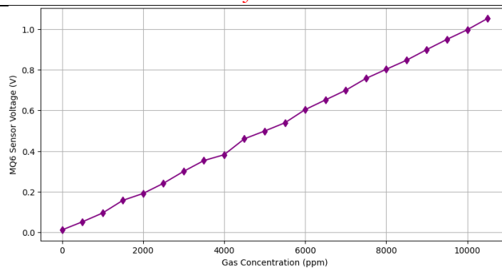
Figure 17. MQ6 Sensor Voltage vs. Gas Concentration.
