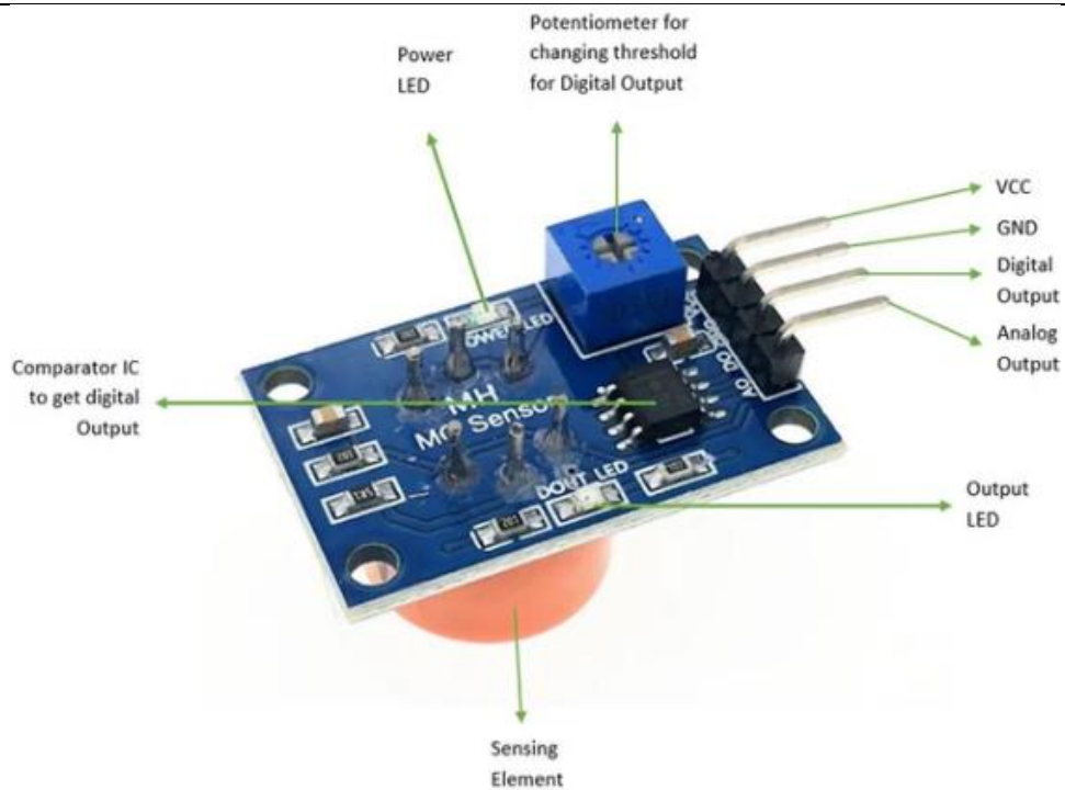
Figure 4. MQ gas sensor module with labeled components.
