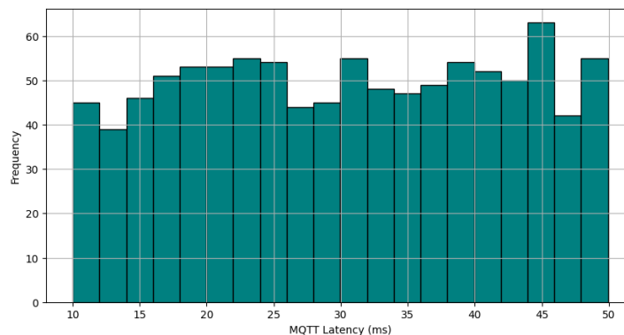
Figure 18. Histogram of MQTT Message Latencies
