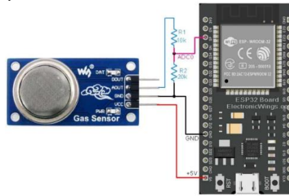
Figure 7. Interfacing the MQ6 sensor module with the ESP32 microcontroller
