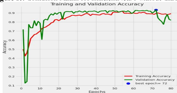
Figure 11. Training and Validation accuracy on EfficientNetB6 without CLAHE
