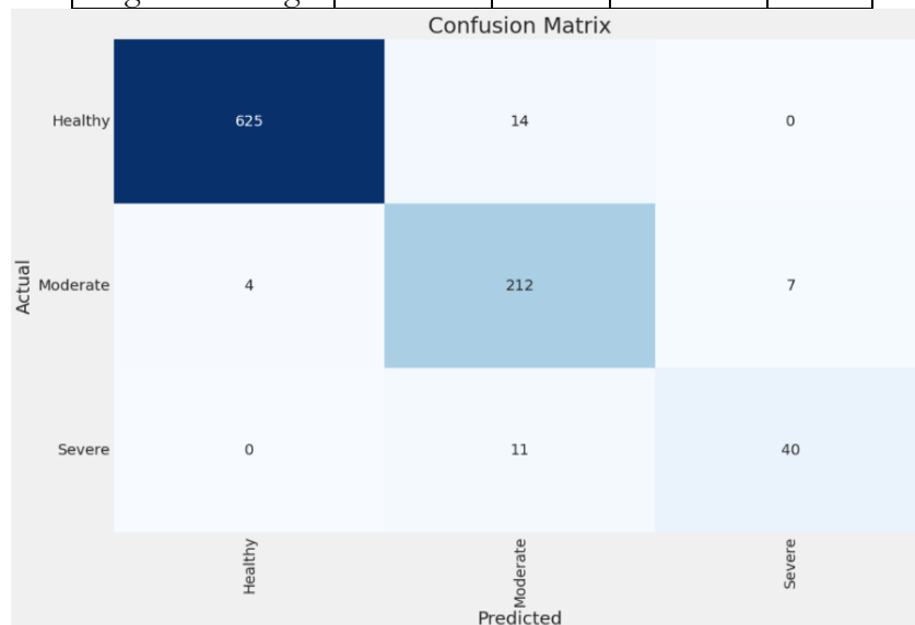
Figure 7. Confusion Matrix for EfficientNetB6 with CLAHE.
