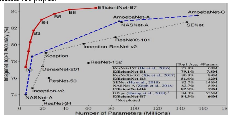
Figure 6. Model size vs ImageNet Accuracy.
