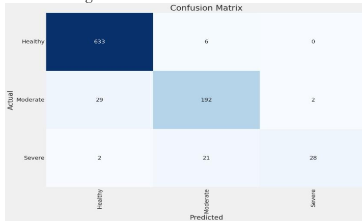
Figure 10. Confusion Matrix for EfficientNetB6 without CLAHE.
