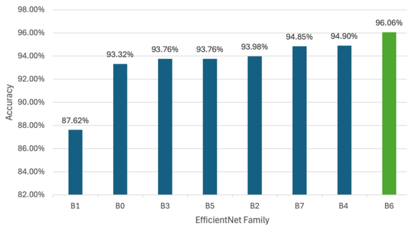
Figure 13. Performance Comparison amongst all EfficientNet Models.
