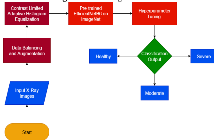
Figure 2. Flow Diagram of methodology.
