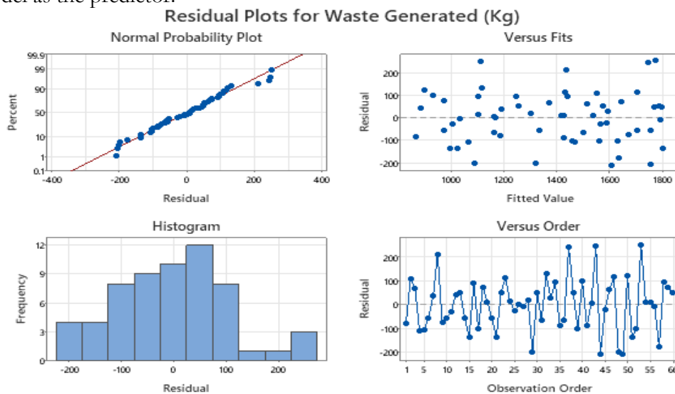
Figure 5. Residual Plots for valid inference
