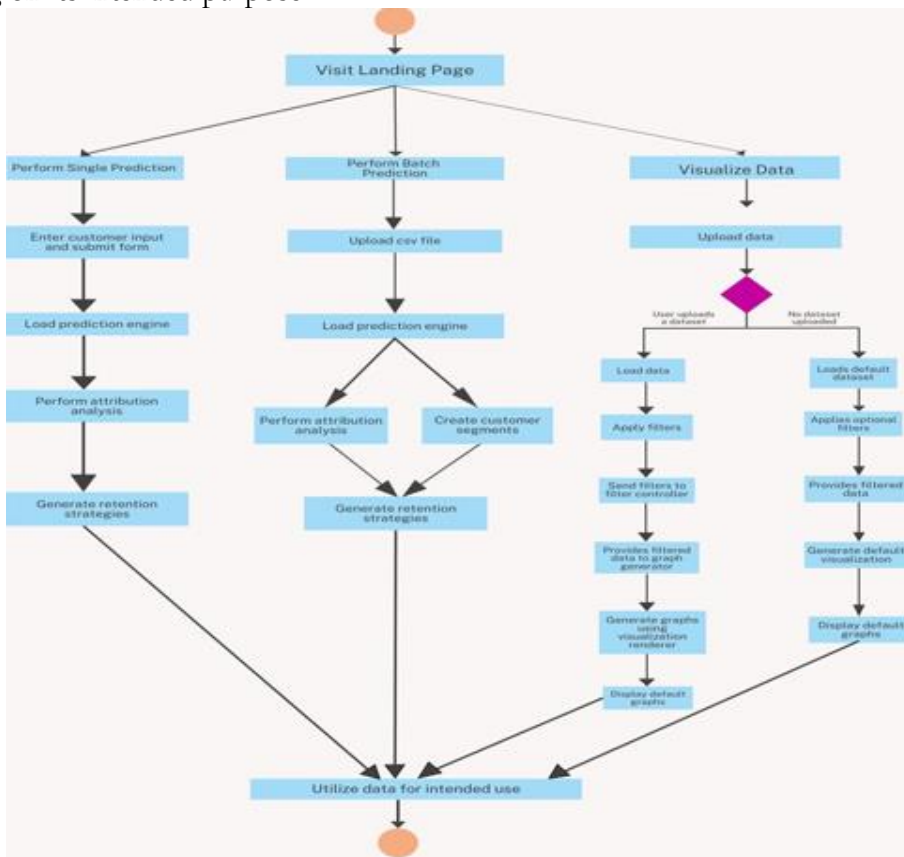
Figure 10. Workflow of TeleChurnAI
