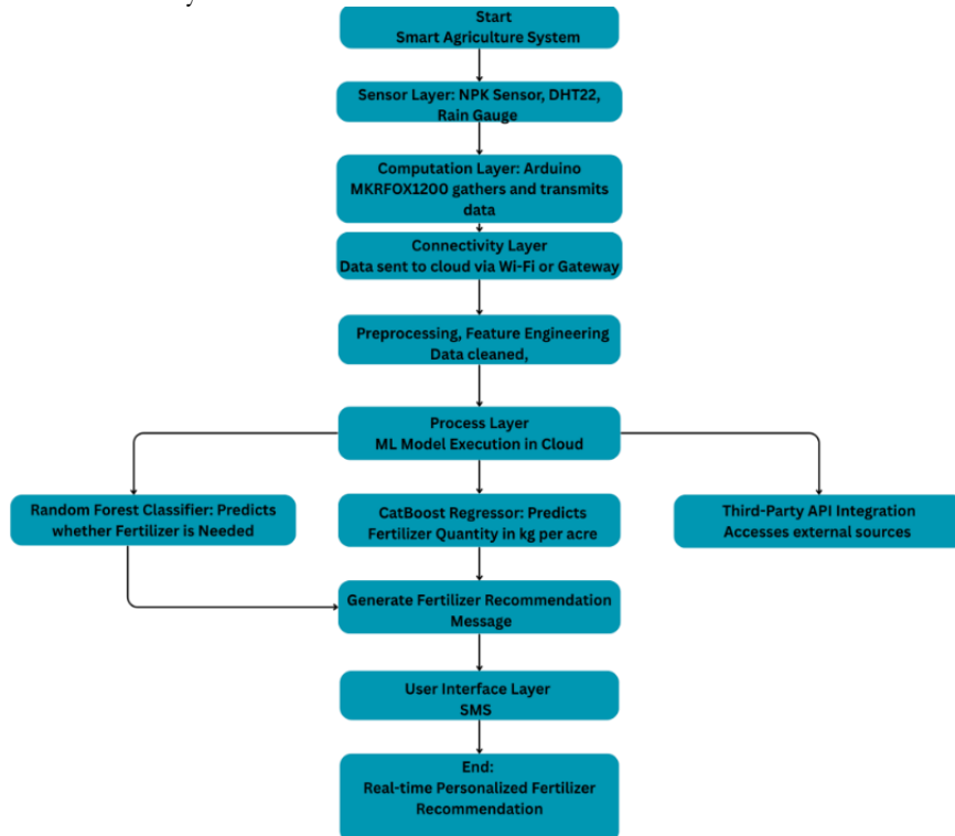
Figure 5. Architecture of a Smart Agriculture System for Real-Time Fertilizer Recommendation Using Machine Learning”
