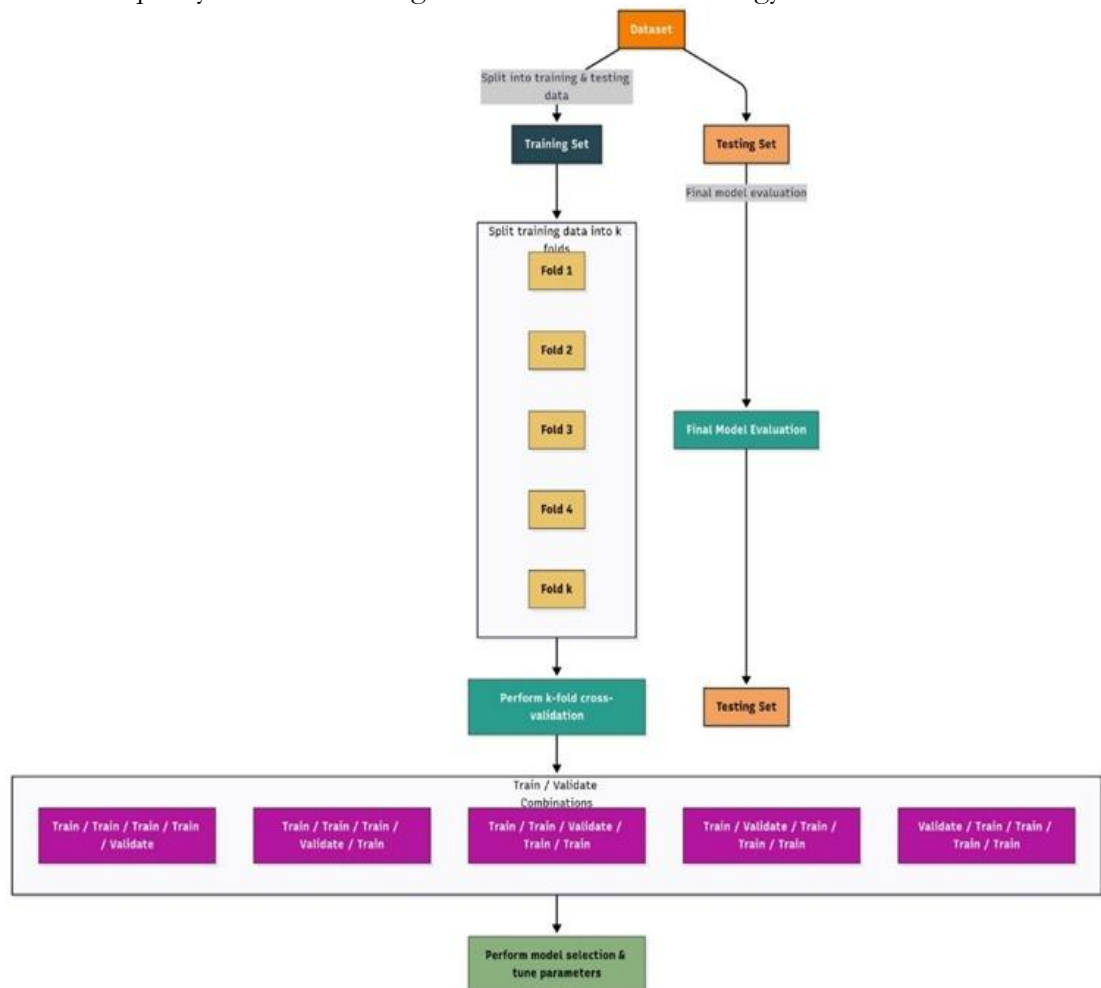
Figure 4. K-Fold Cross Validation Workflow for Model Training, Validation, and Final Evaluation
