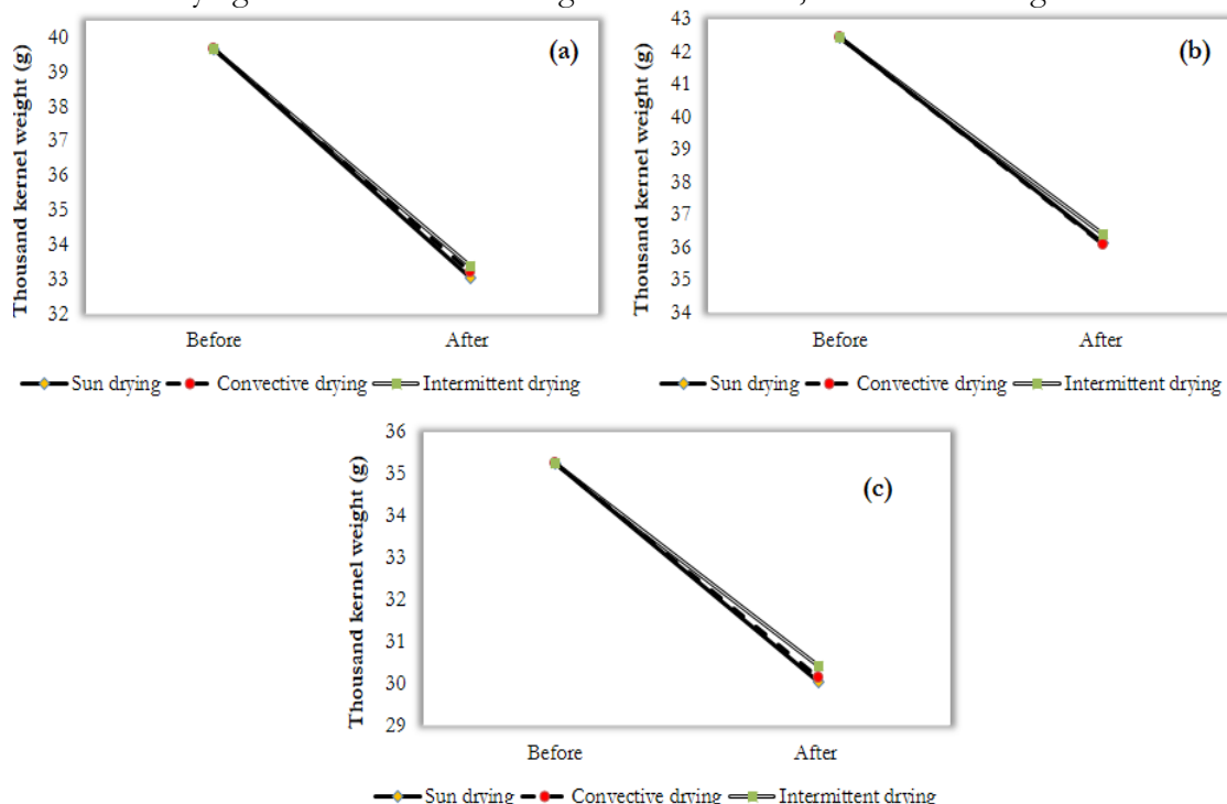
Figure 7. Variation in thousand kernel weight (g) of varieties TD-1 (a), Imdaad-2005 (b) and Sindhu (c) under different drying methods.
