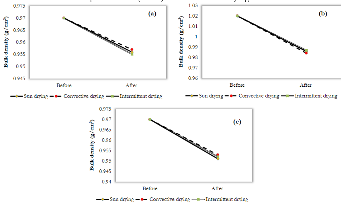
Figure 9. Variation in bulk density (g/cm 3 ) of varieties TD-1 (a), Imdaad-2005 (b) and Sindhu (c) under different drying methods.
