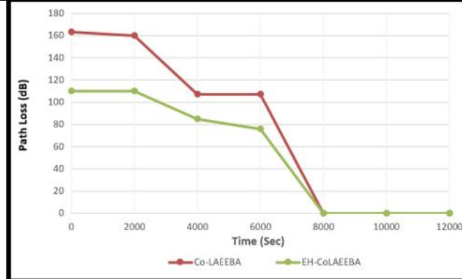
Figure 5. Path-loss (dB) vs. time (s)
