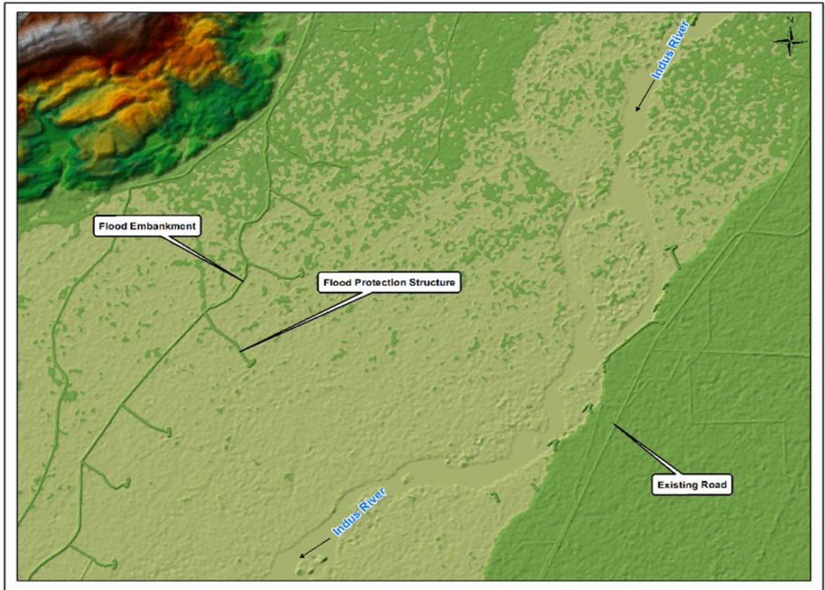
Figure 5. TIN-derived surface from calibrated SRTM data showing major flood-protection structures along the Indus River.
