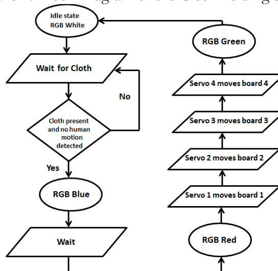
Figure 3. Workflow of the Automated Cloth-Folding System
