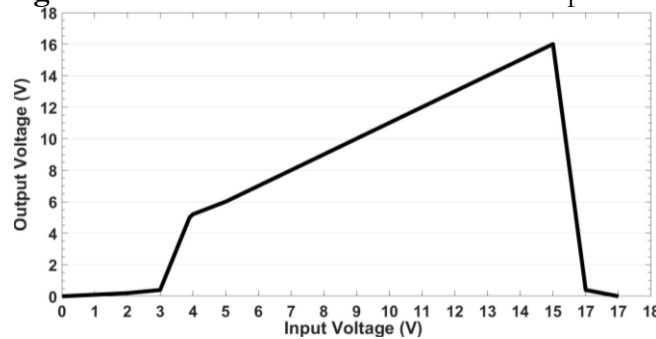
Figure 6. Protection Circuit Board Input Vs Output Voltage
