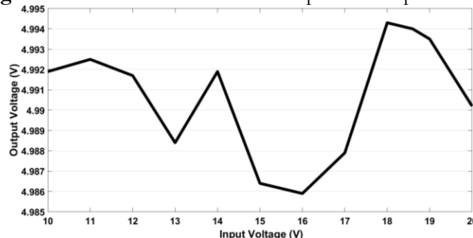
Figure 7. Output Voltage vs Input Voltage for 5V Voltage Regulator
