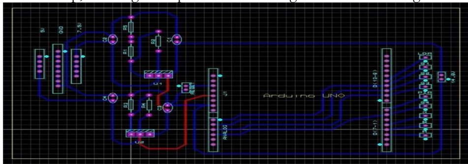
Figure 4. PCB Layout
