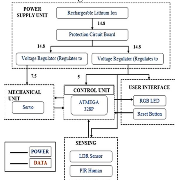
Figure 2. Block Diagram of the Cloth-Folding System
