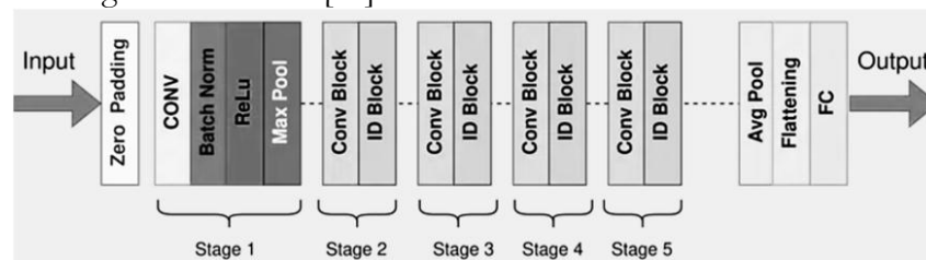
Figure 3. ResNet-50 Architecture.
