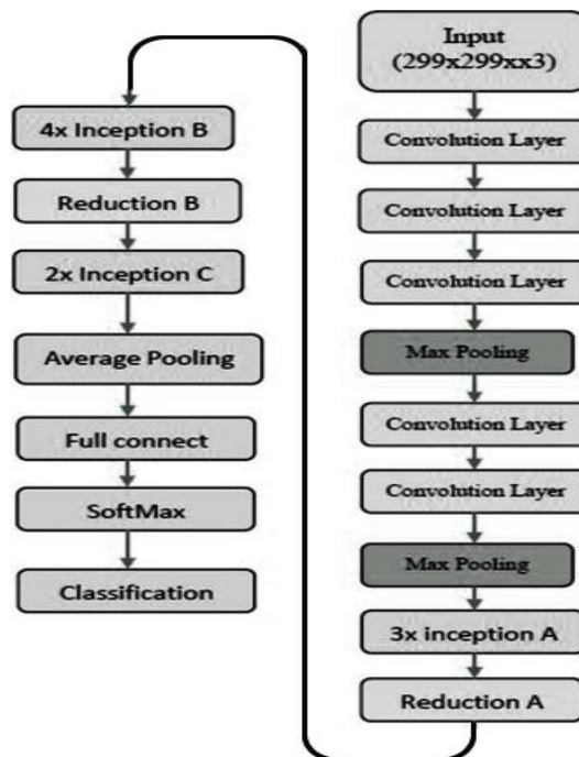
Figure 4. InceptionV3 Architecture
