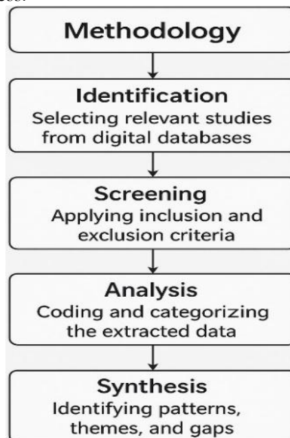
Figure 4. Research Methodology
