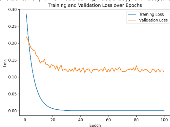
Figure 5. Training and Validation Loss Across Epochs
