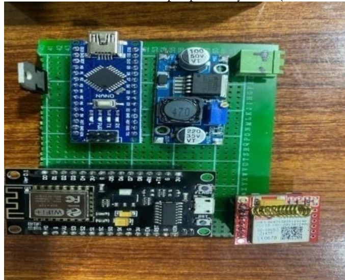
Figure 2. Hardware prototype of the proposed car battery theft prevention system
