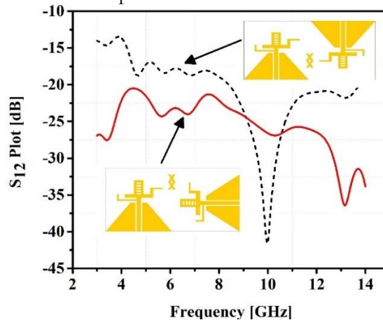
Figure 7. MIMO antenna orientation effect on mutual coupling.
