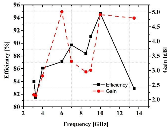
Figure 16. Gain and efficiency of the proposed antenna.
