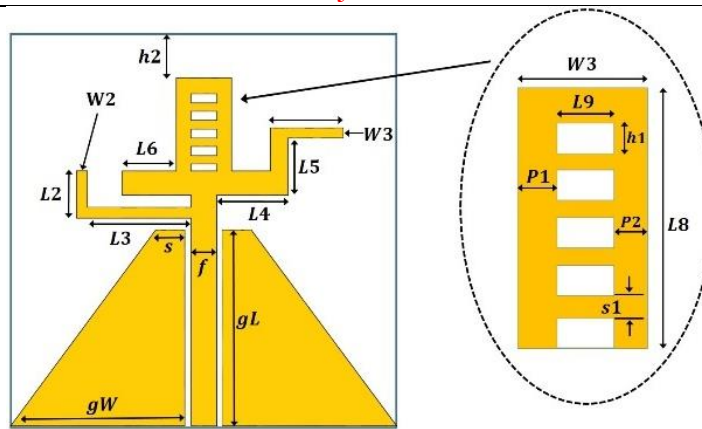
Figure 3. Labeled design of a proposed antenna.
