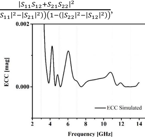
Figure 14. ECC of the proposed antenna.
