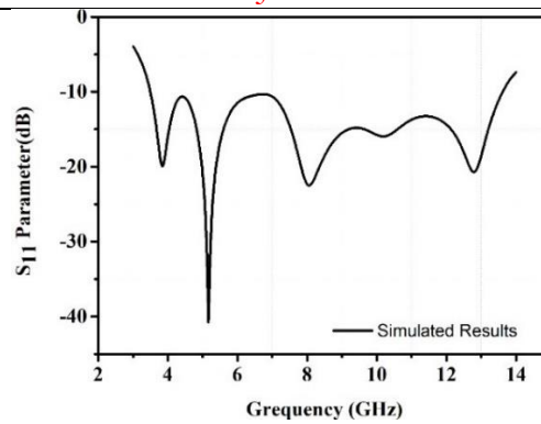
Figure 8. Simulated S-parameter of the proposed antenna.
