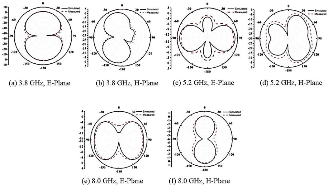
Figure 12. The simulated radiation pattern of the proposed antenna.
