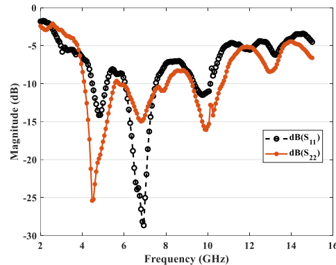
Figure 9. Measured S-parameters of proposed MIMO antennas.
