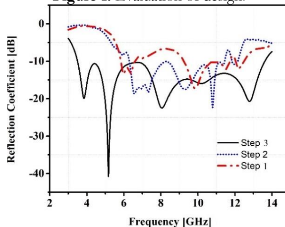
Figure 2. S-parameters of in-step antennas.
