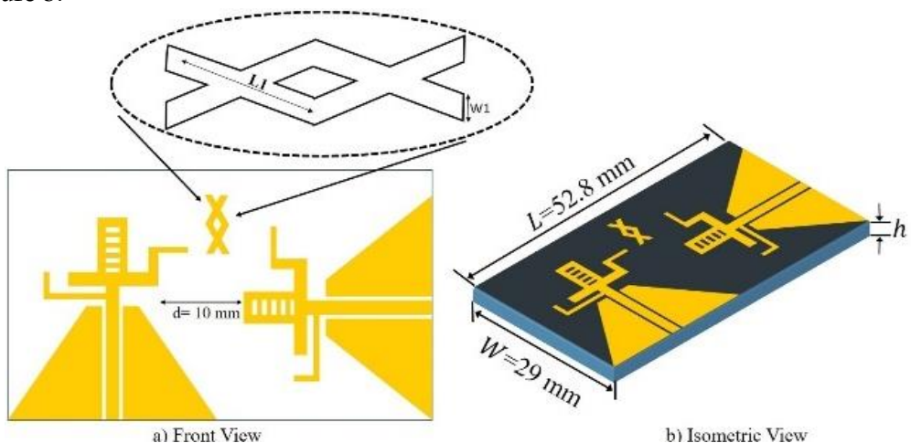
Figure 4. MIMO Antenna configuration.
