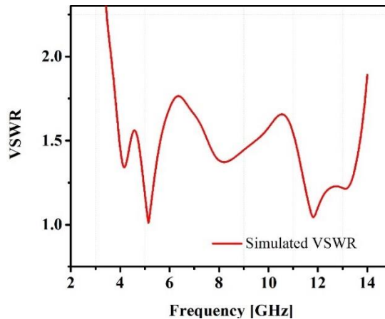
Figure 10. Simulated VSWR of a proposed antenna.
