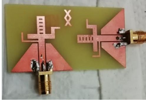
Figure 5. Fabricated MIMO antenna prototype.
