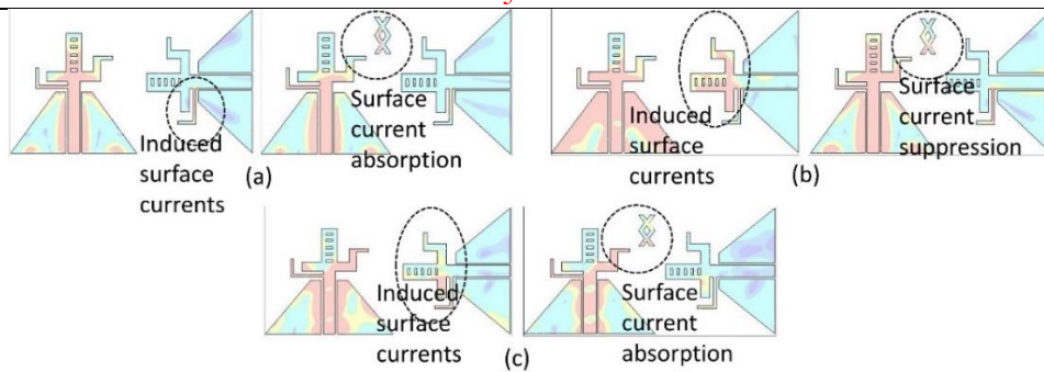
Figure 11. The current distribution of proposed MIMO at different frequencies. (a) 3.8 GHz (b) 5.2 GHz and (c) 8.0 GHz
