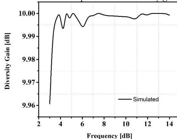
Figure 15. Diversity gains of the proposed antenna.
