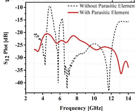
Figure 6. Effect of parasitic elements on mutual coupling.
